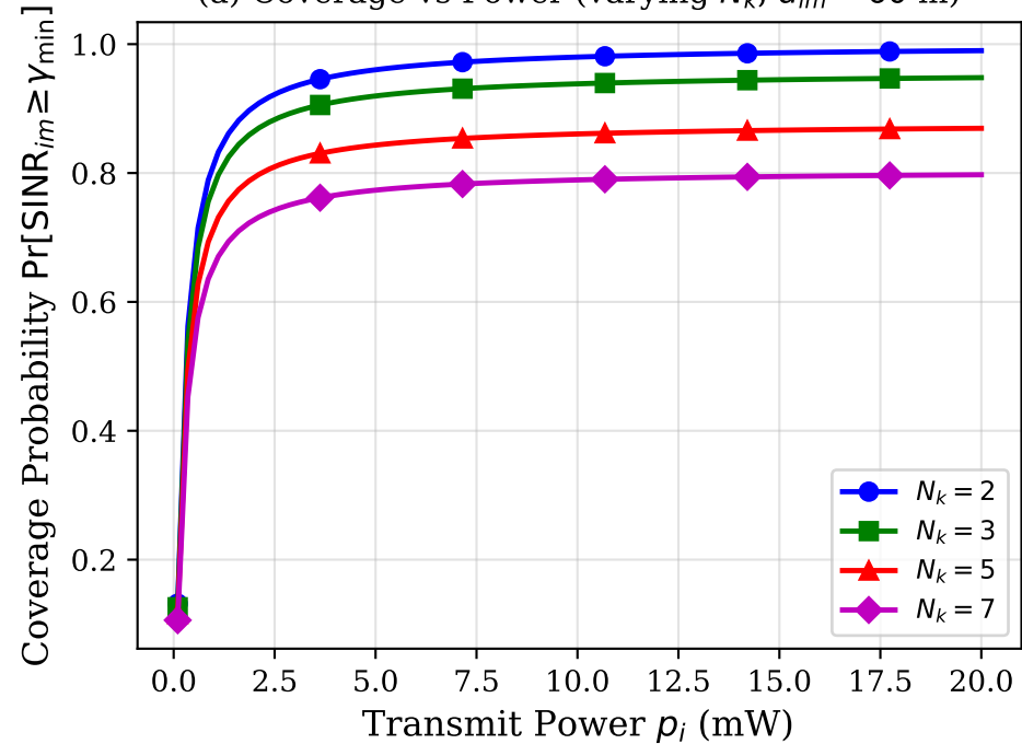
(a) Coverage vs Power (varying N_k , d_{im} = 60 m)
