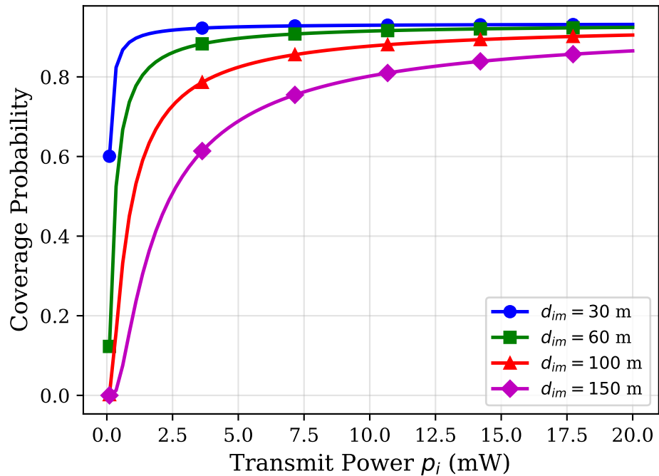
(b) Coverage vs Power (varying d_{im} , N_k = 4 )
