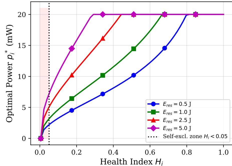
(a) Self-Exclusion: p_i^* \rightarrow 0 as H_i \rightarrow 0
