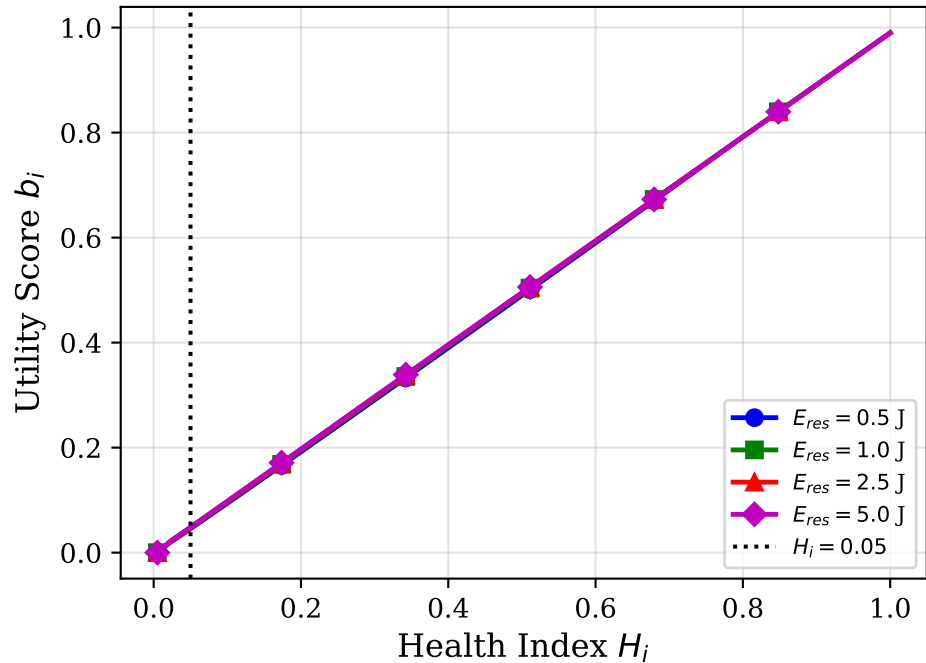
(b) Utility Score b_i \rightarrow 0 as H_i \rightarrow 0
