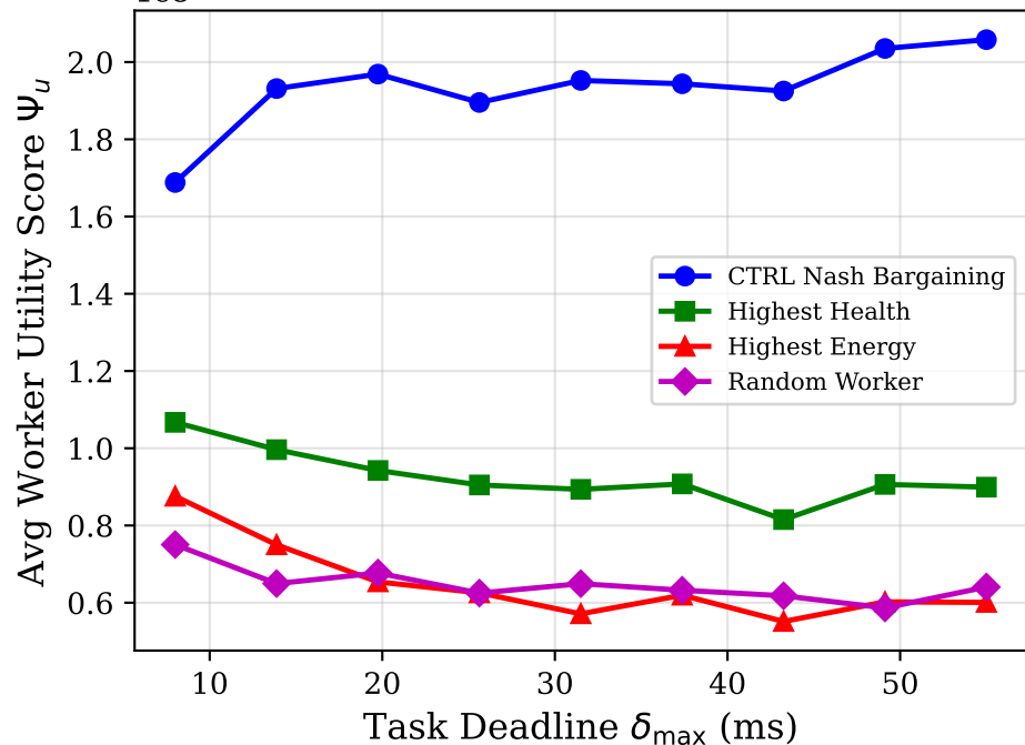
(b) Worker Utility Score vs Deadline
