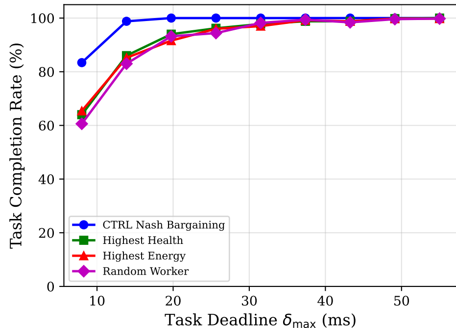
(a) Completion Rate vs Deadline
