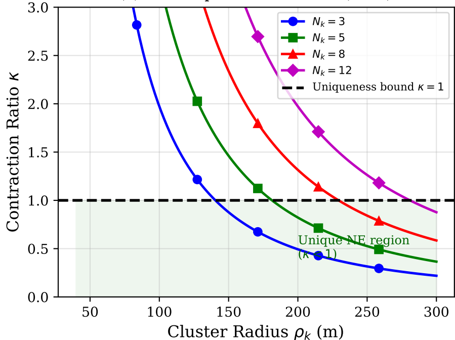
(a) NE Uniqueness Condition ( \kappa < 1 )
