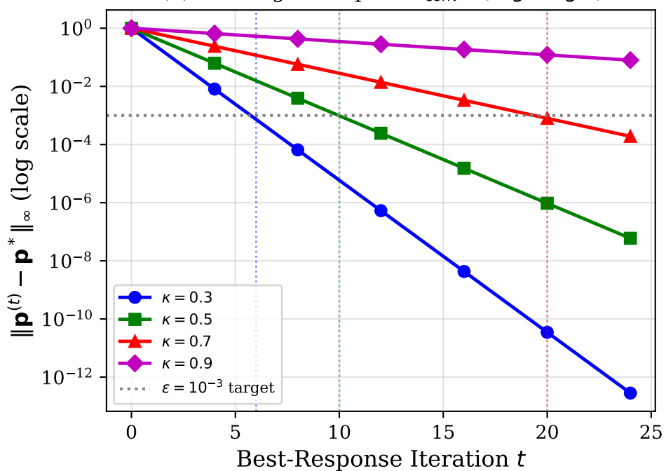
(b) Convergence Speed T_{\text{conv}} = \lceil \log \varepsilon / \log \kappa \rceil
