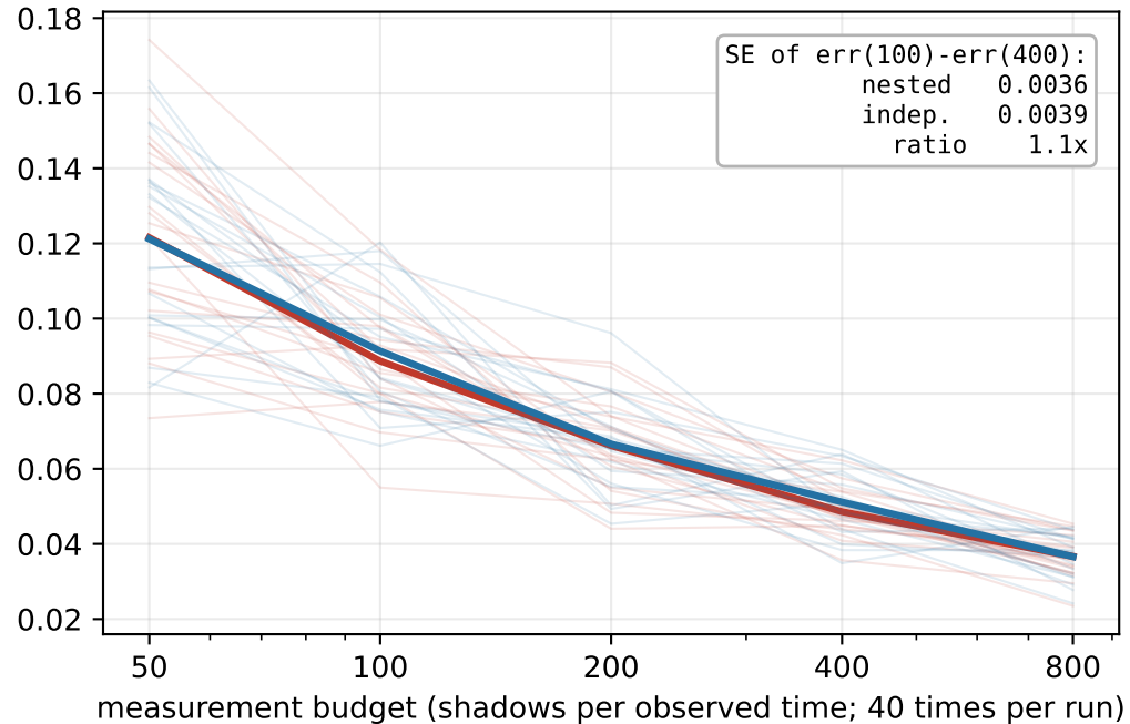
GP reconstruction
