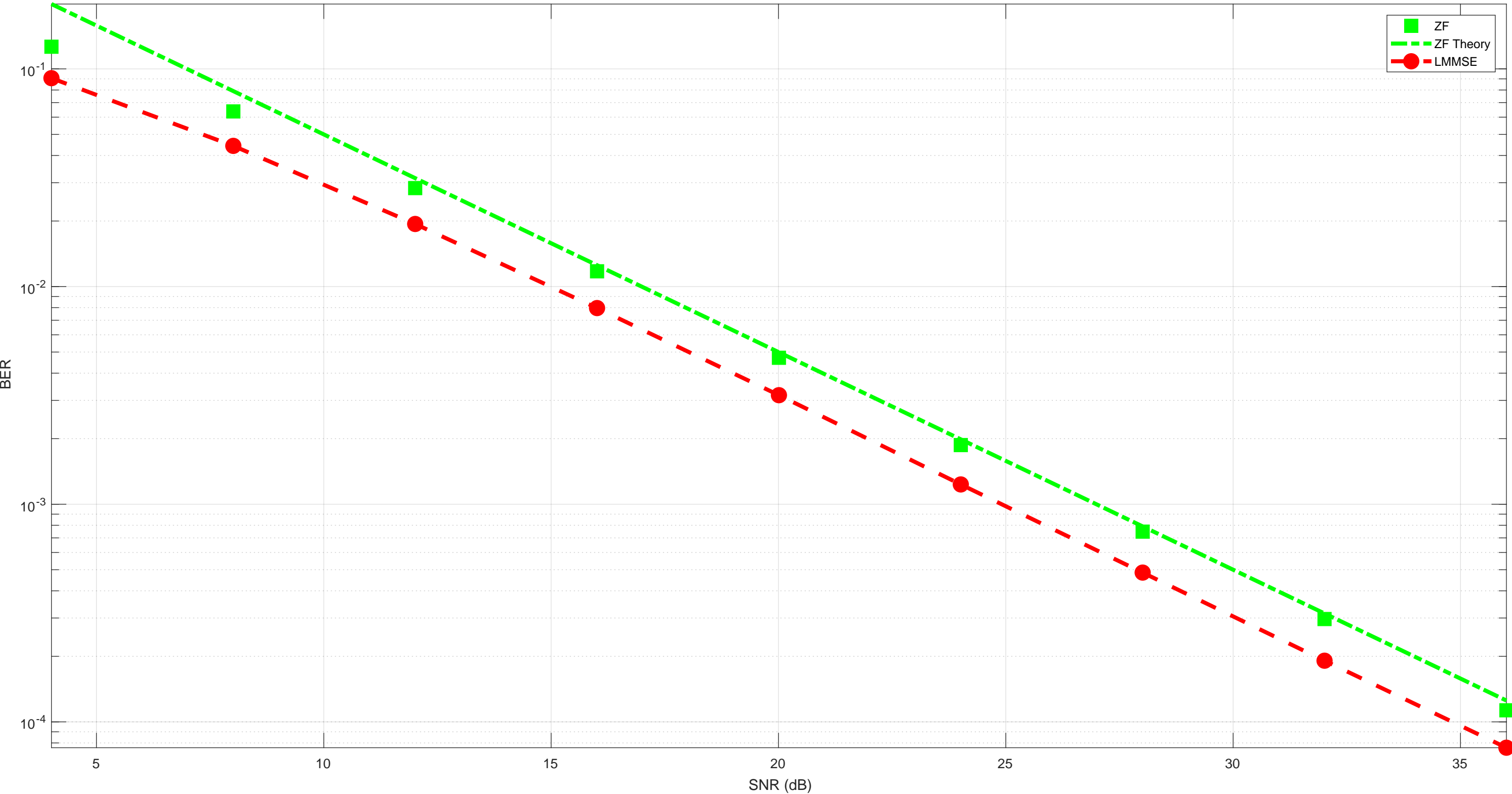
BER vs SNR(dB) for MIMO ZF/ MMSE Receivers
