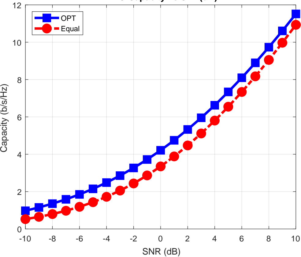
MIMO Capacity vs SNR(dB)
