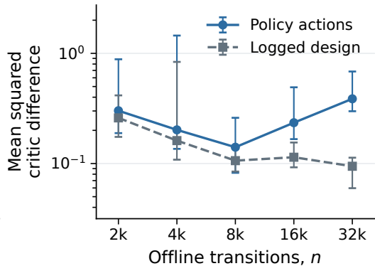
(b) Nyström KRR
