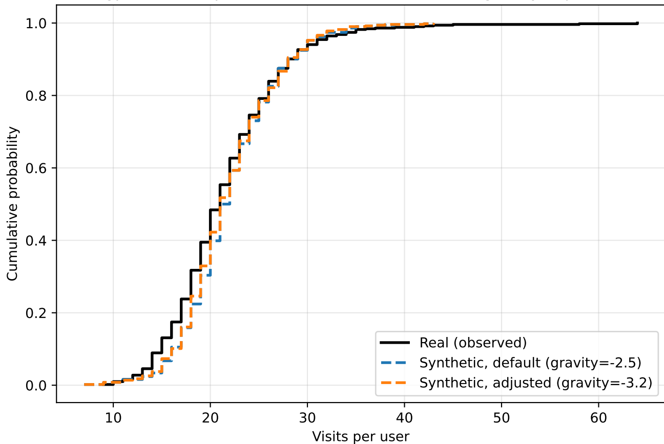
gparis: visits-per-user distribution, default vs. gravity-adjusted
