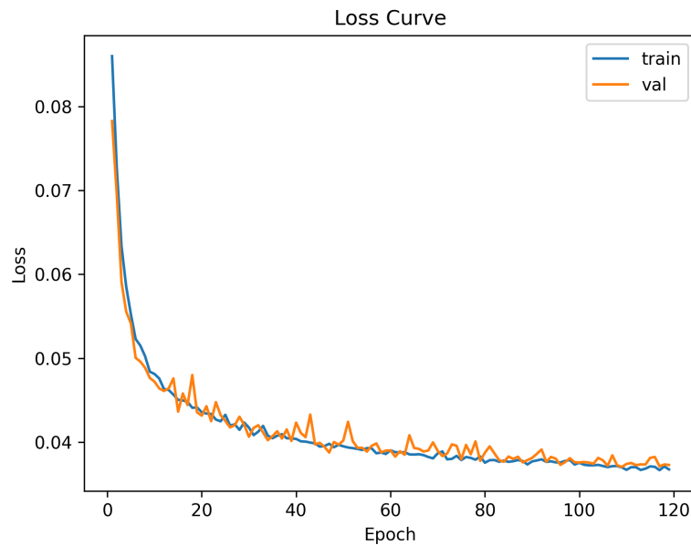
Figure 2: Loss curve for the forward noising U-Net. Both the training and validation loss stabilize at around epoch 100. The loss starts out jittery but it around epoch 120 it is stable. The generalization error is almost zero as well.
