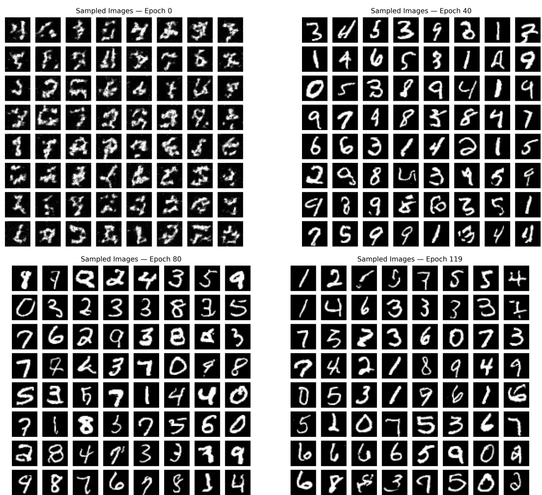
Figure 3: Samples generated at different epochs. The digits are formed around epoch 40 and there are tiny improvements as the epochs progress.
