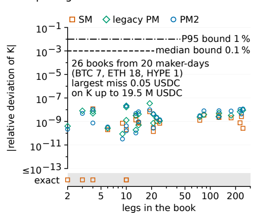
b opening books
