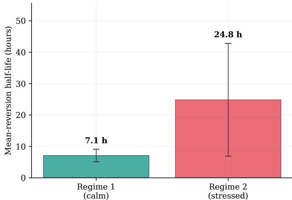
(b) Implied half-life \tau = \ln 0.5 / \ln |\phi_k| , delta-method 95% CI
