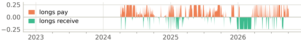
Bitfinex BVIV-perp funding (% per 8h, daily mean; cap \pm 0.25\% )
