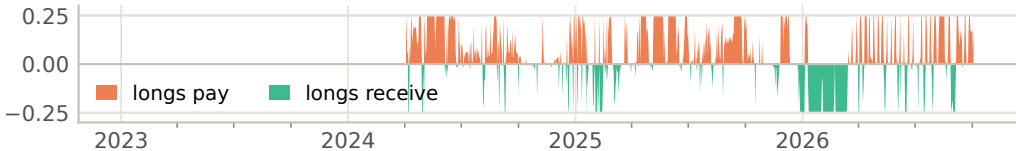
Bitfinex BVIV-perp funding (% per 8h, daily mean; cap \pm 0.25\% )
