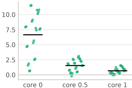
Timing value by core hedge
