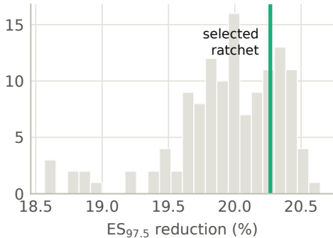
ES reduction: ratchet vs. its placebos
