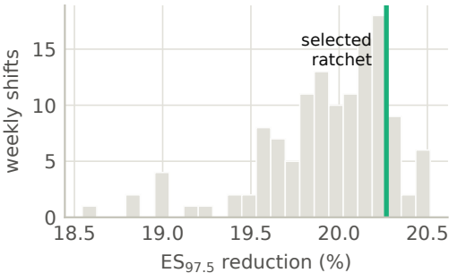
ES reduction: ratchet vs. its placebos
