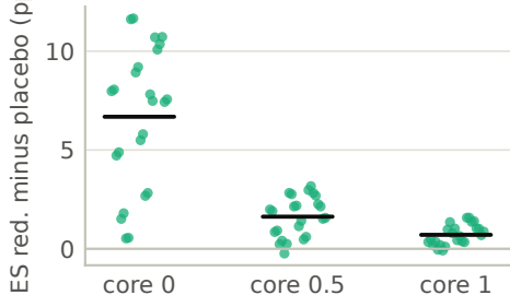
Timing value by core hedge
