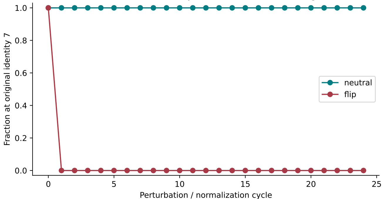
Normal-form recovery versus cross-class damage
