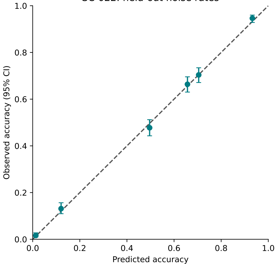
SC-022: held-out noise rates
