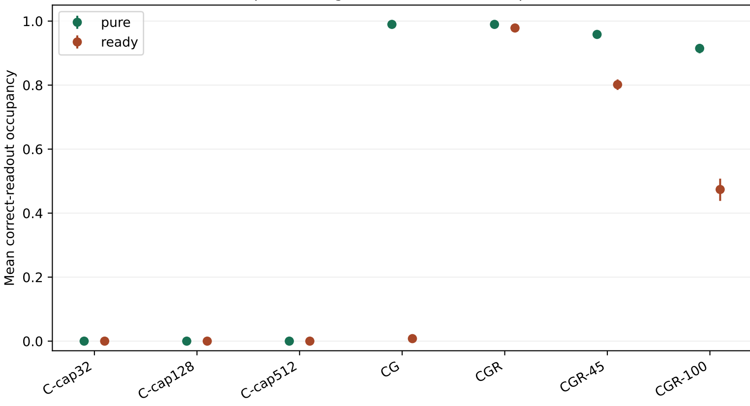
SC-026: steps 1 through 8000, seed-bootstrap 95% intervals
