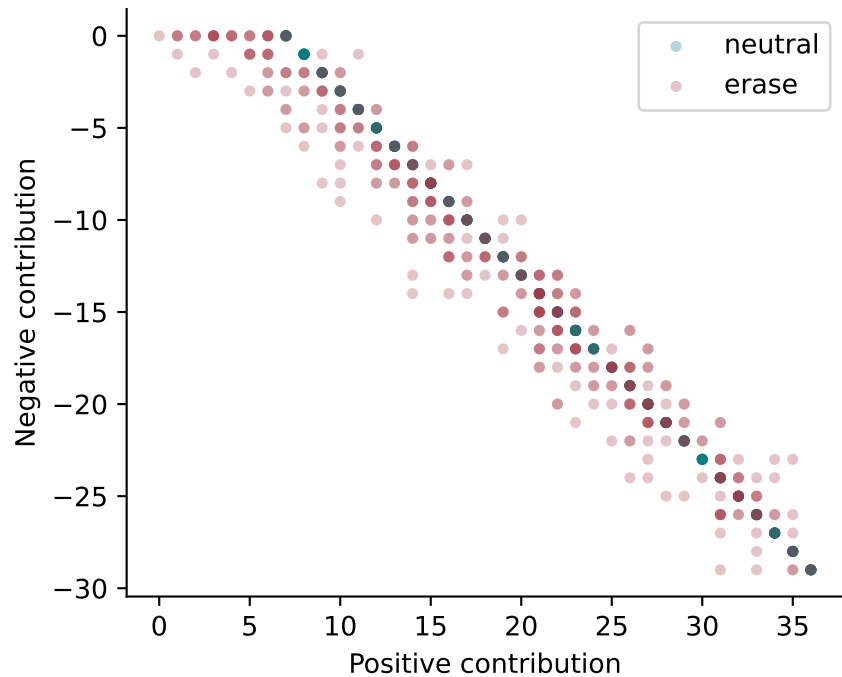
Covariance across independent microstates
