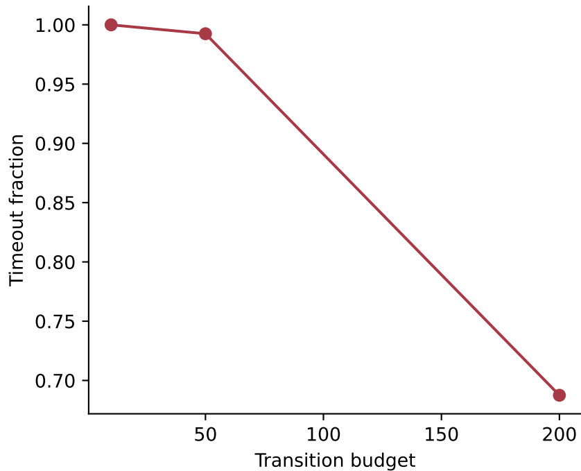
32-region local dynamics
