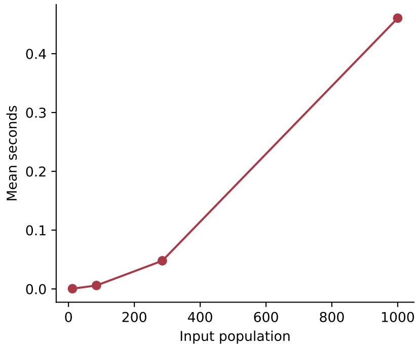
Observed runtime (including hashing)
