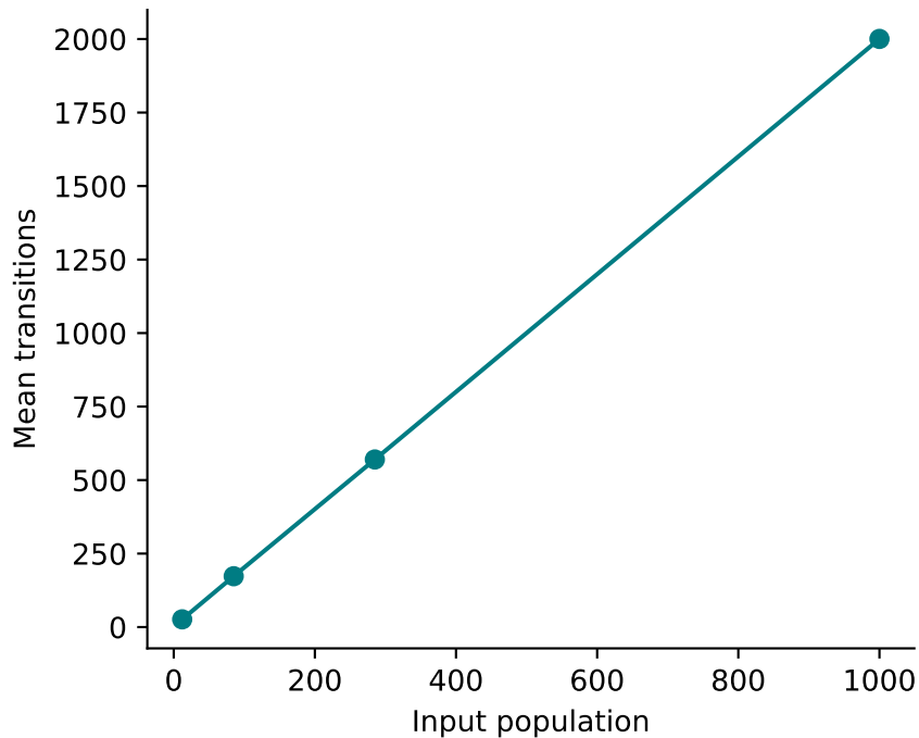
Unary addition work
