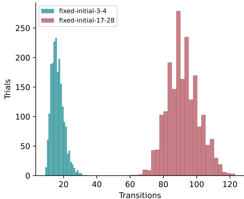
Identical initial states, varying schedules
