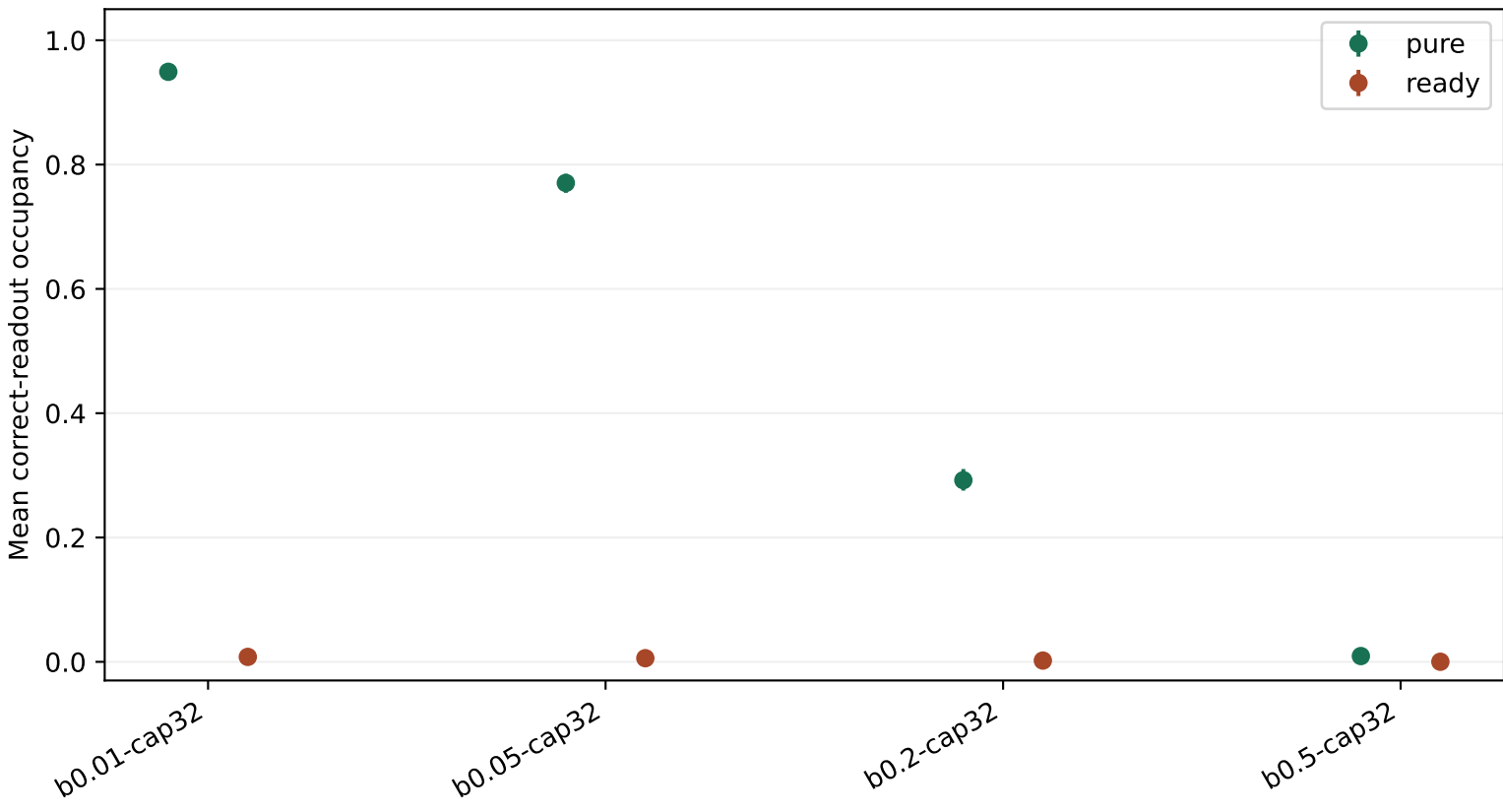
SC-027R: steps 4001 through 8000, seed-bootstrap 95% intervals
