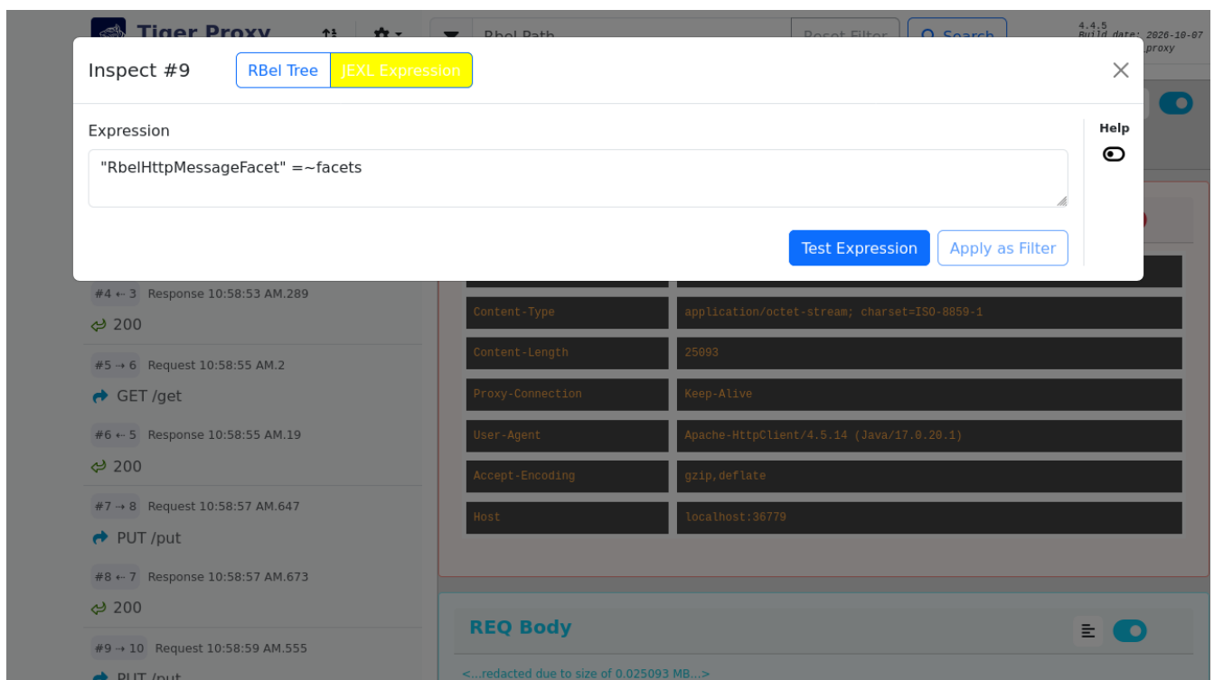
Figure 74. JEXL Debugging
