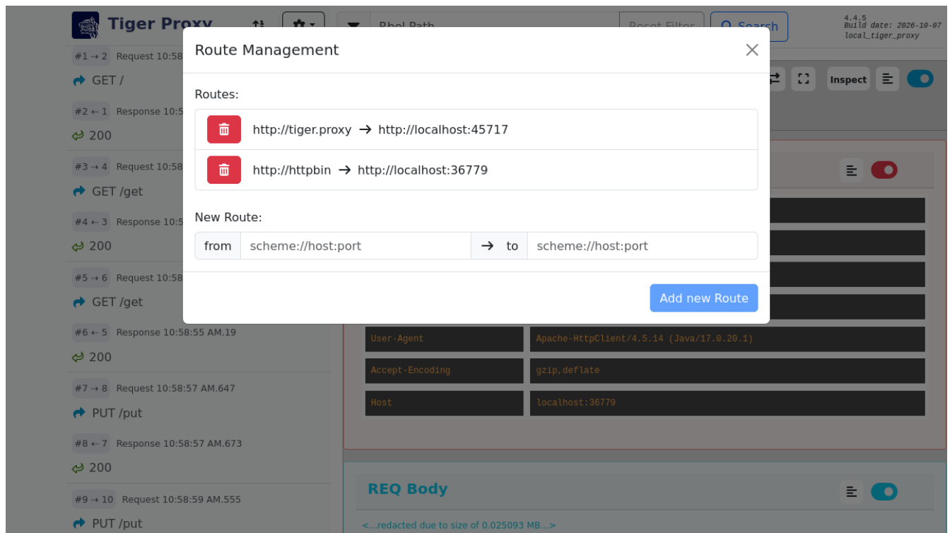
Figure 75. Route Management
