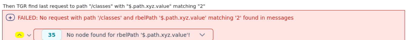
Figure 38. Up Button
