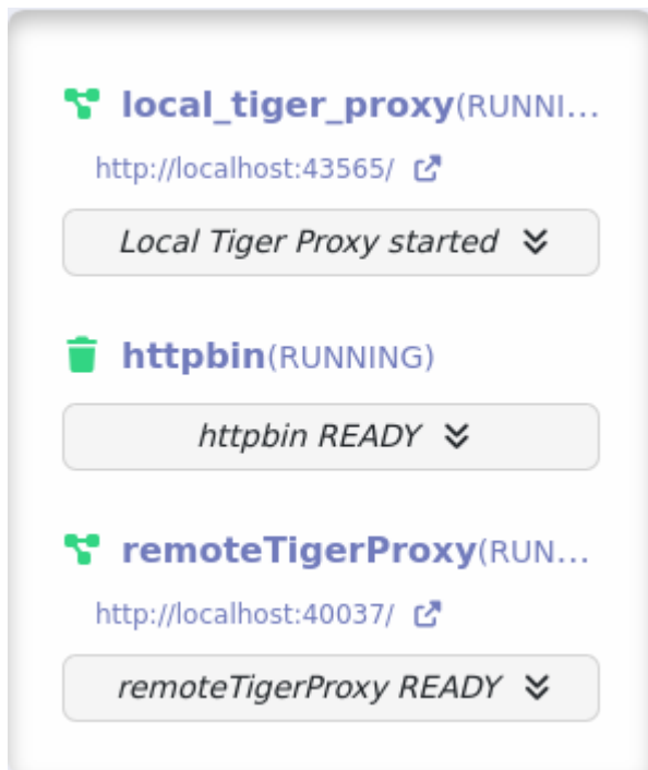
Figure 27. server box
