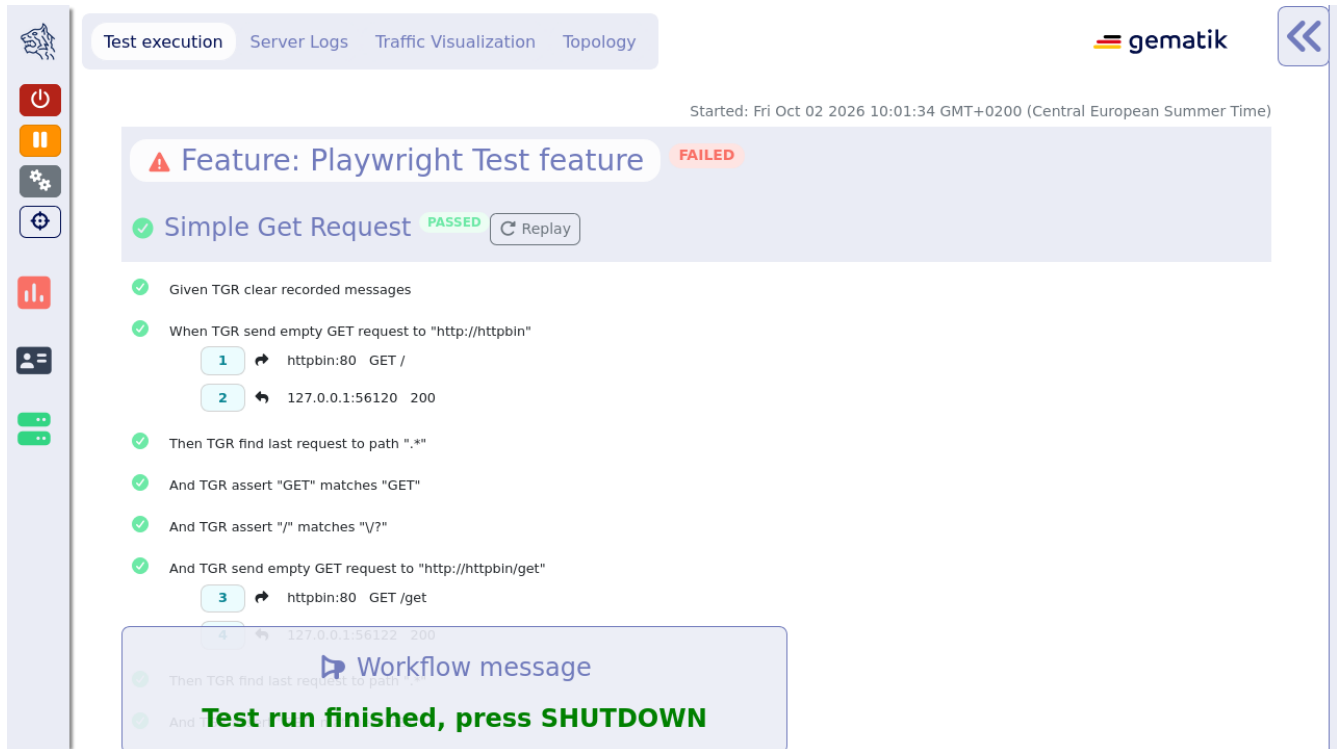
Figure 19. Workflow UI
