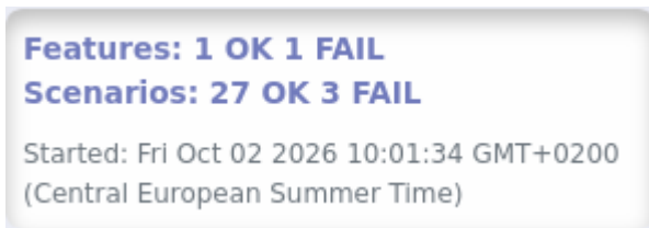
Figure 25. status box
