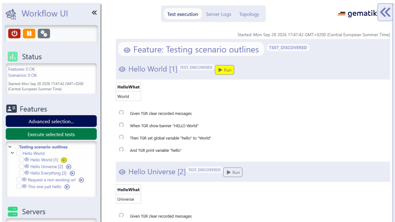
Figure 52. Play Buttons
