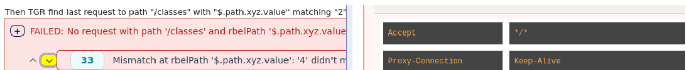
Figure 37. Down Button
