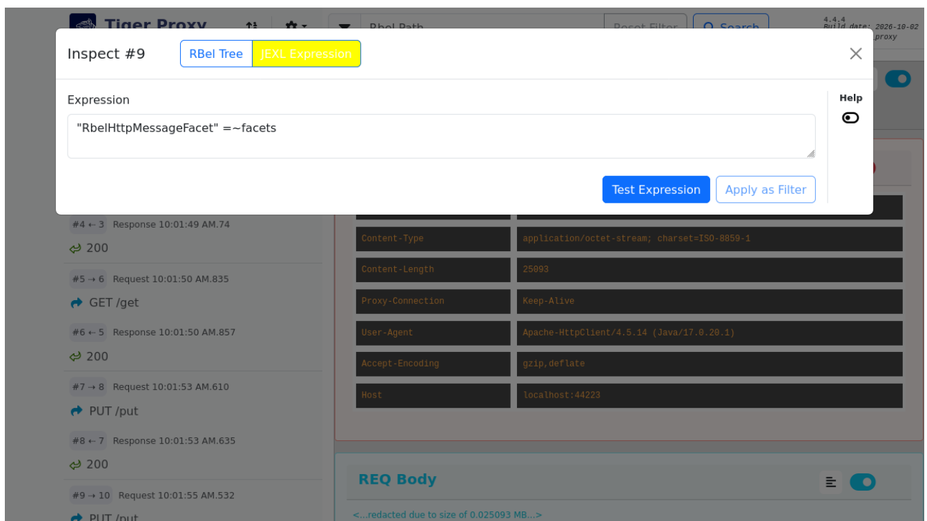
Figure 74. JEXL Debugging
