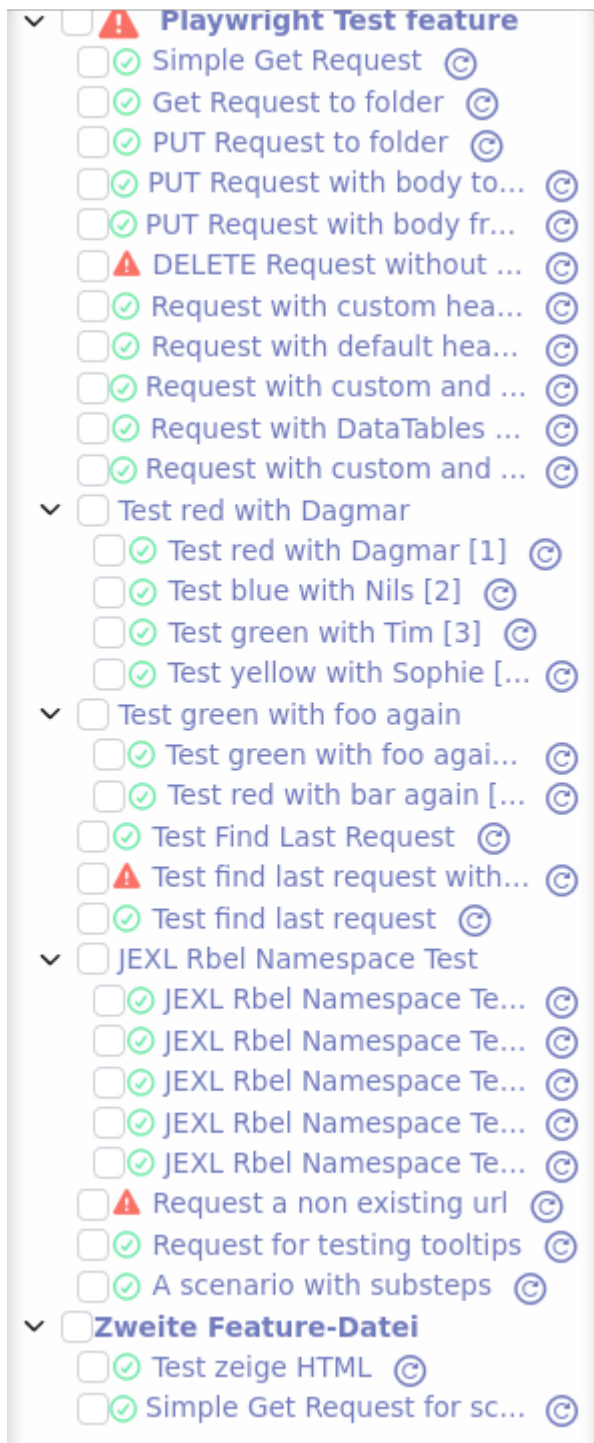
Figure 26. feature box
