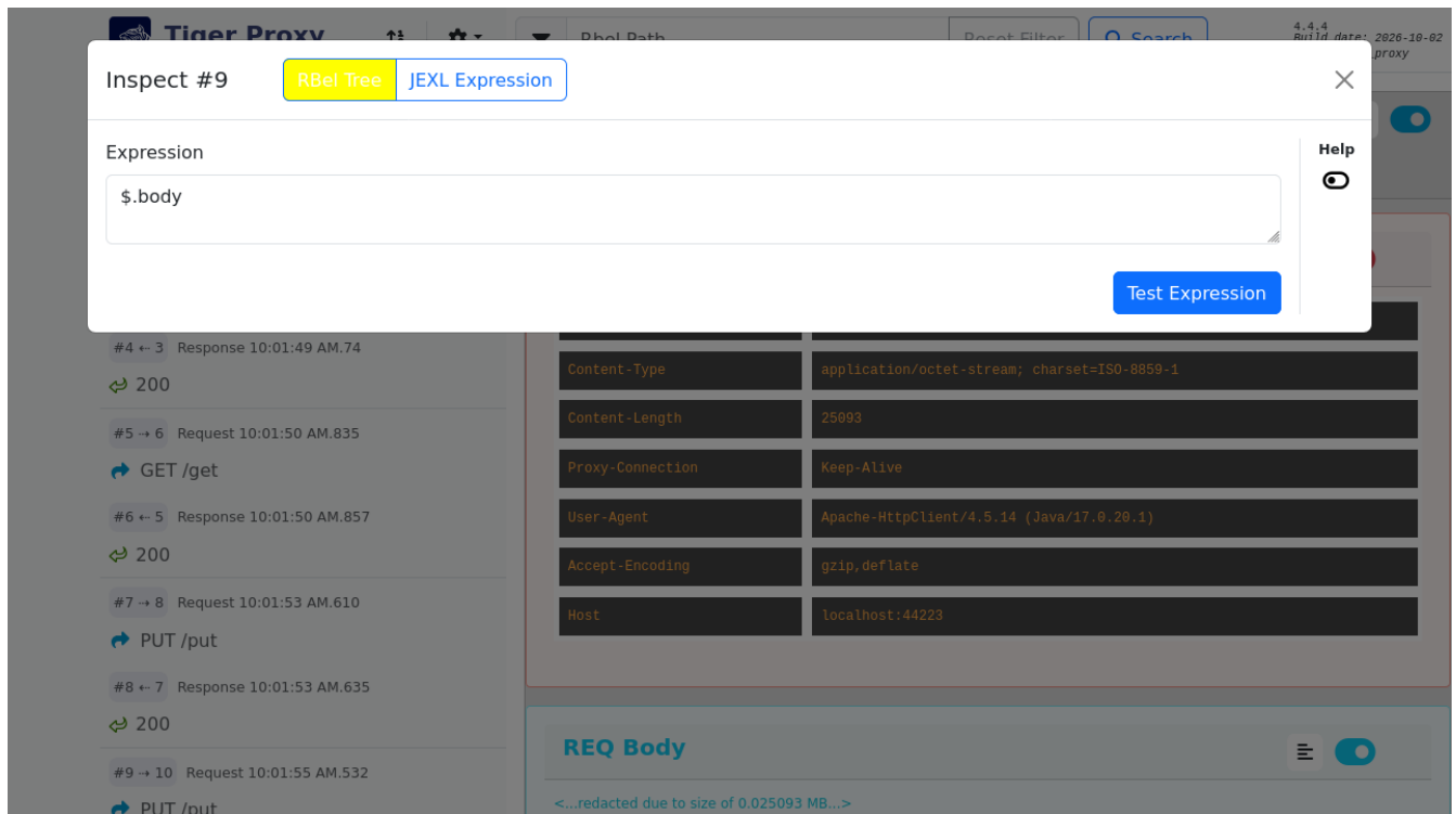
Figure 73. RBel-Path
