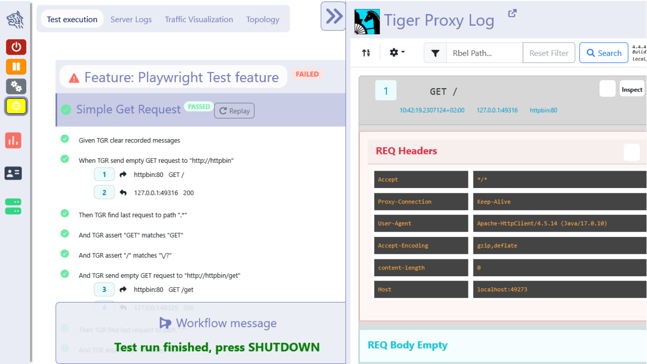
Figure 48. Scoping active
