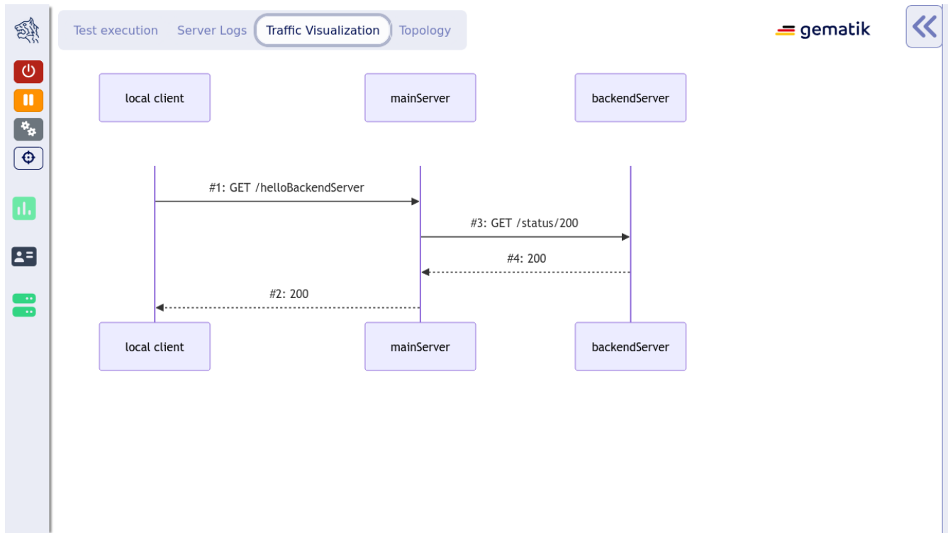
Figure 51. Traffic Visualization
