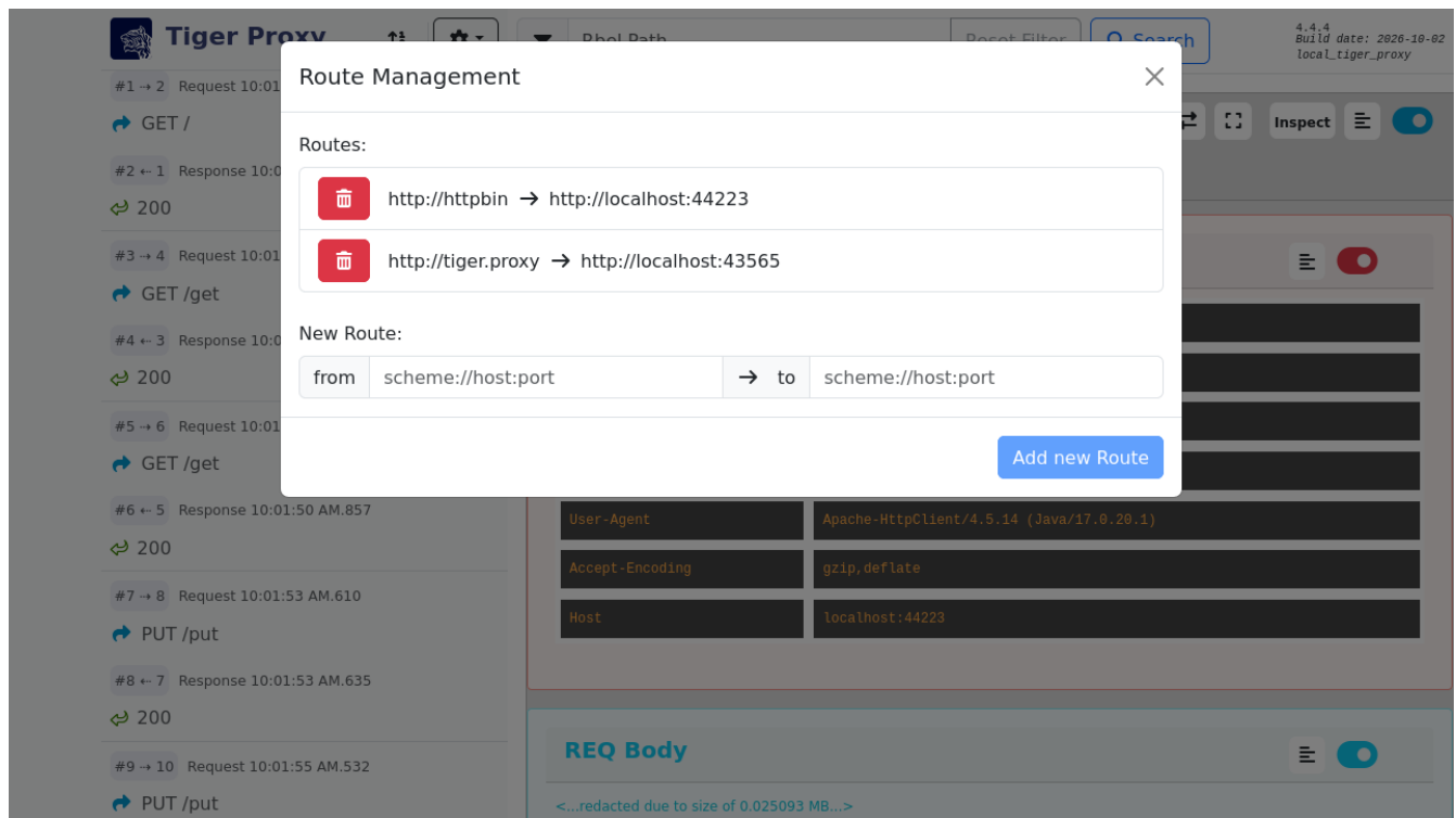
Figure 75. Route Managment
