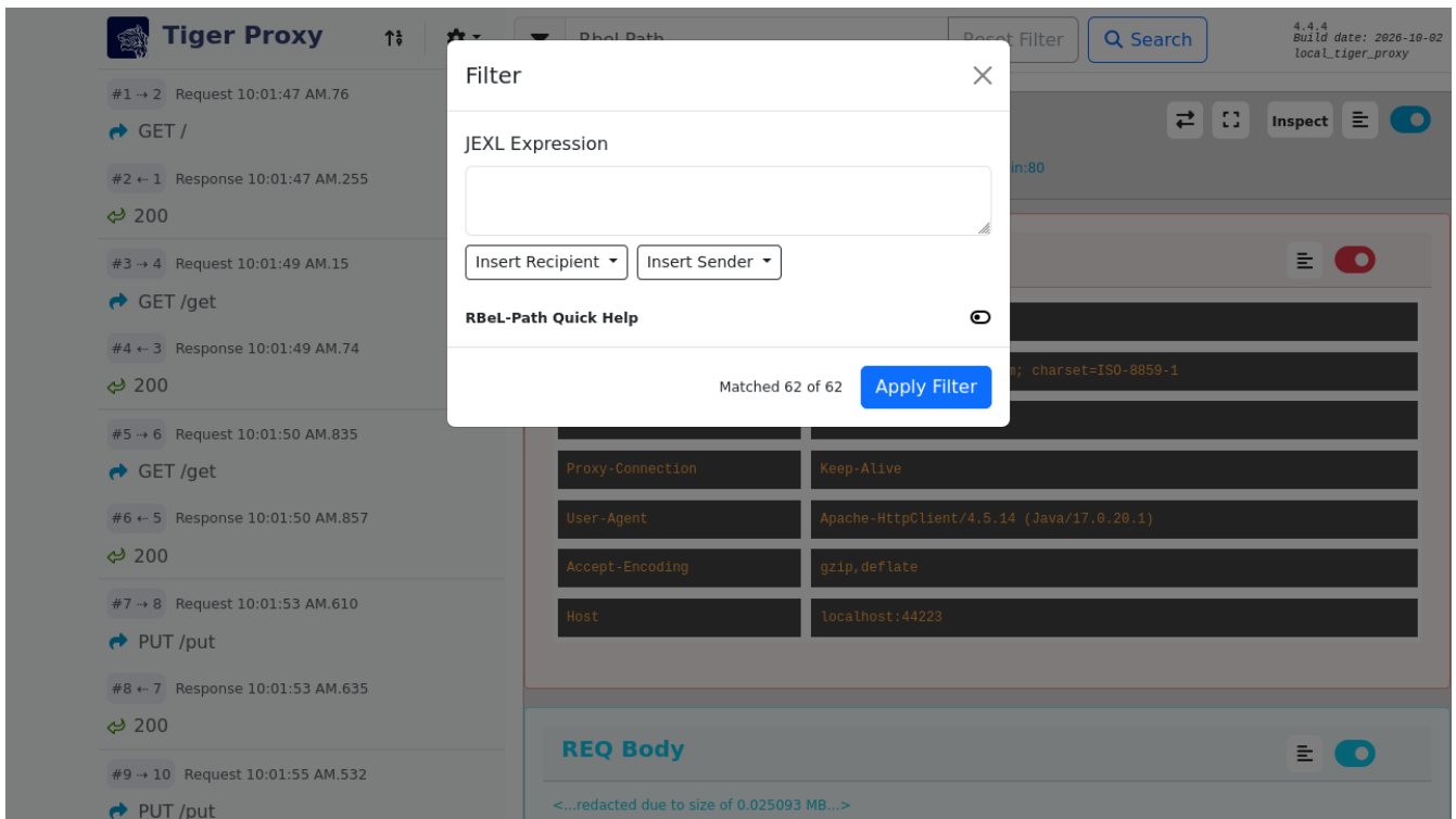
Figure 71. Filter Management
