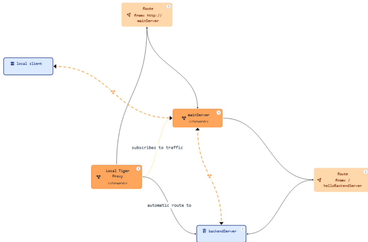
Figure 63. Topology diagram with additional edges between local client, mainServer and backendServer
