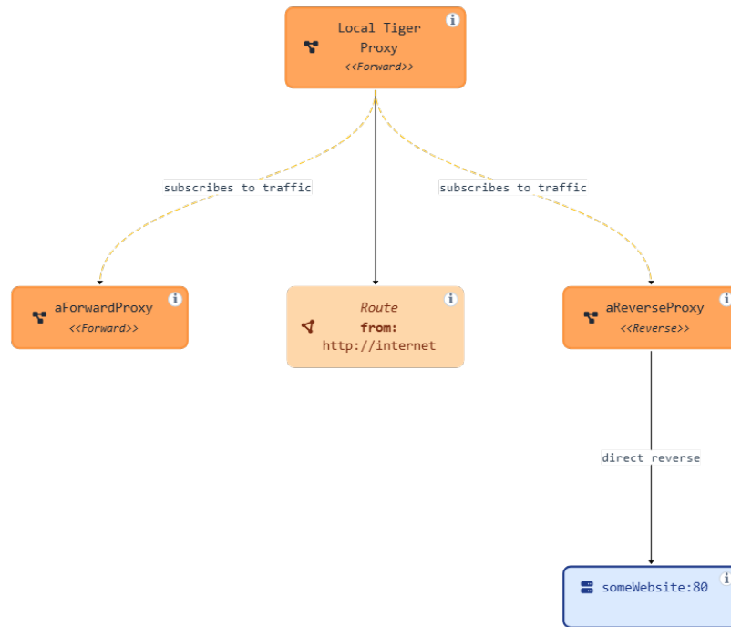
Figure 56. Local tiger proxy subscribes to traffic from two other proxies. One is configured as a reverse proxy. A route to an external URL is also configured.
