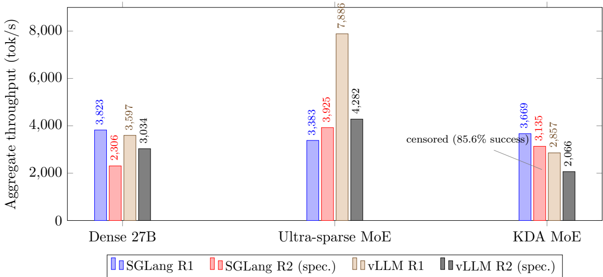
Figure 2: Aggregate throughput of the three battles (values from Tables 4–7). R2 denotes speculative decoding enabled. The vLLM R2 bar on the KDA model is a censored measurement (85.6% success; work truncated at 623k tokens, Section 4).
