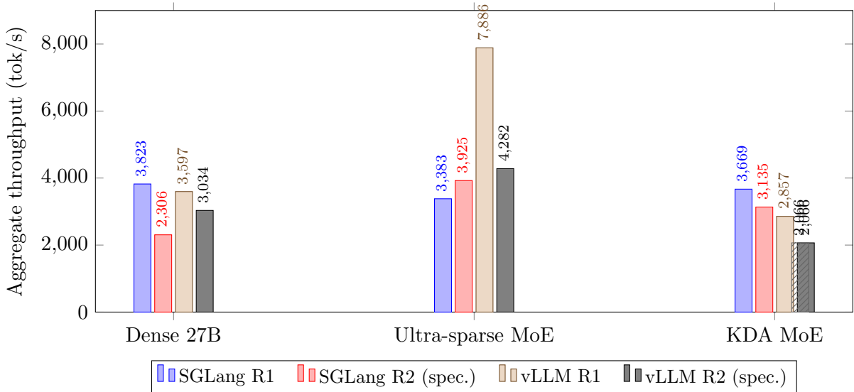
Figure 2: Aggregate throughput of the three battles (values from Tables 4–7). R2 denotes speculative decoding enabled. The hatched bar (vLLM R2 on the KDA model) is a censored measurement: 85.6% success, work truncated at 623k tokens (Section 4).
