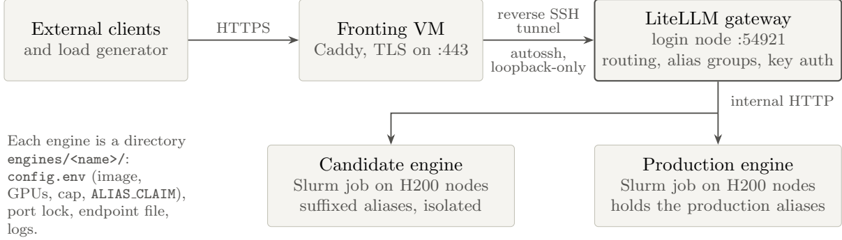
Figure 1: Request path from external clients through the gateway to engine jobs. A candidate engine registers only suffixed aliases, so it receives benchmark traffic without claiming production names; switching which engine holds the production aliases is a two-line ALIAS_CLAIM edit plus a gateway restart (Section 3).
