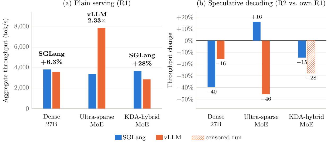
Figure 2: The three battles at a glance (values from Tables 4–7). (a) Plain-serving throughput; the label above each pair names the winner and its margin. (b) Change in aggregate throughput when the checkpoint’s speculative-decoding head is enabled, relative to the same framework’s R1; five of six bars are below zero. SGLang’s dense R2 also includes its automatic cap reduction from 128 to 48 (Section 5.1). The hatched bar is a censored measurement: 85.6% success, work truncated at 623k tokens (Section 4).
