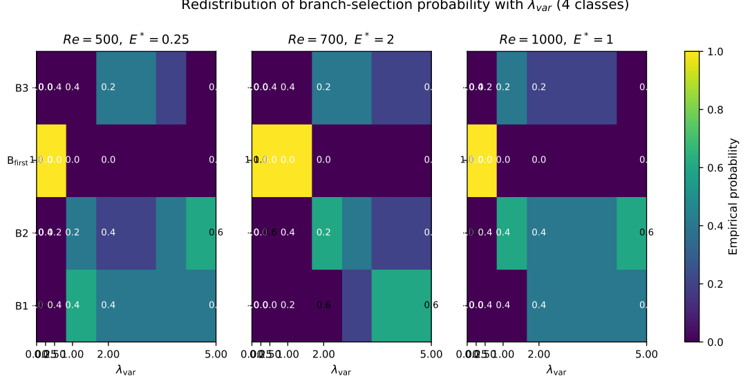
Figure 3: Empirical redistribution of branch-selection frequencies with the variance-regularization weight \lambda_{\text{var}} for three fixed operating conditions. Heatmaps show the four classes B_1 , B_2 , B_{\text{first}} , and B_3 ; cell values are empirical frequencies estimated from five independent realizations per \lambda_{\text{var}} value. 95% Wilson-score confidence intervals are tabulated in Supplementary Sec. S4.
