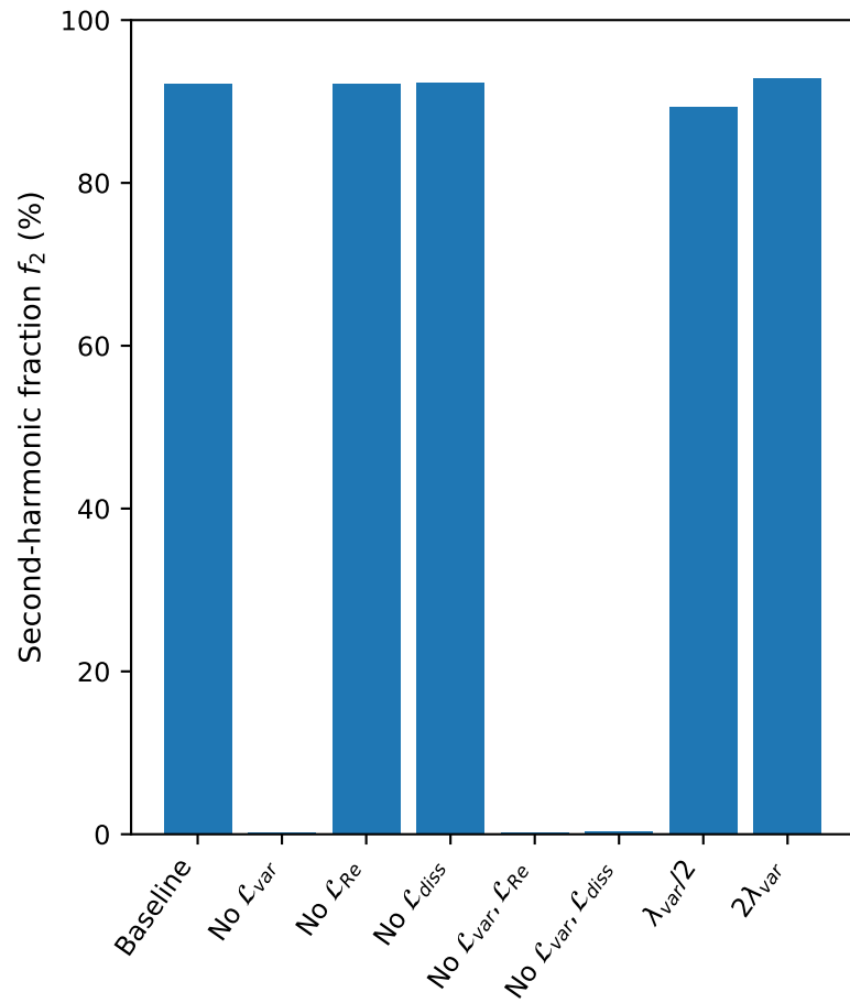
Loss-term ablation at Re = 500 : removing \mathcal{L}_{var} selects the first-harmonic branch B_{\text{first}}
