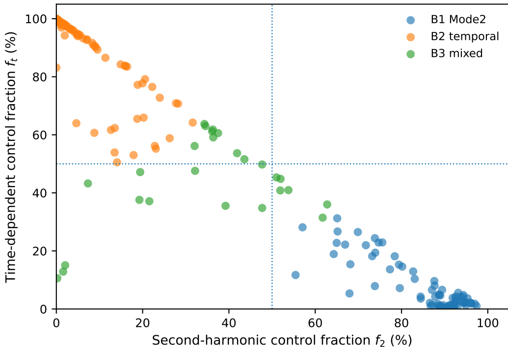
Empirical output-space separation of the three branch classes
