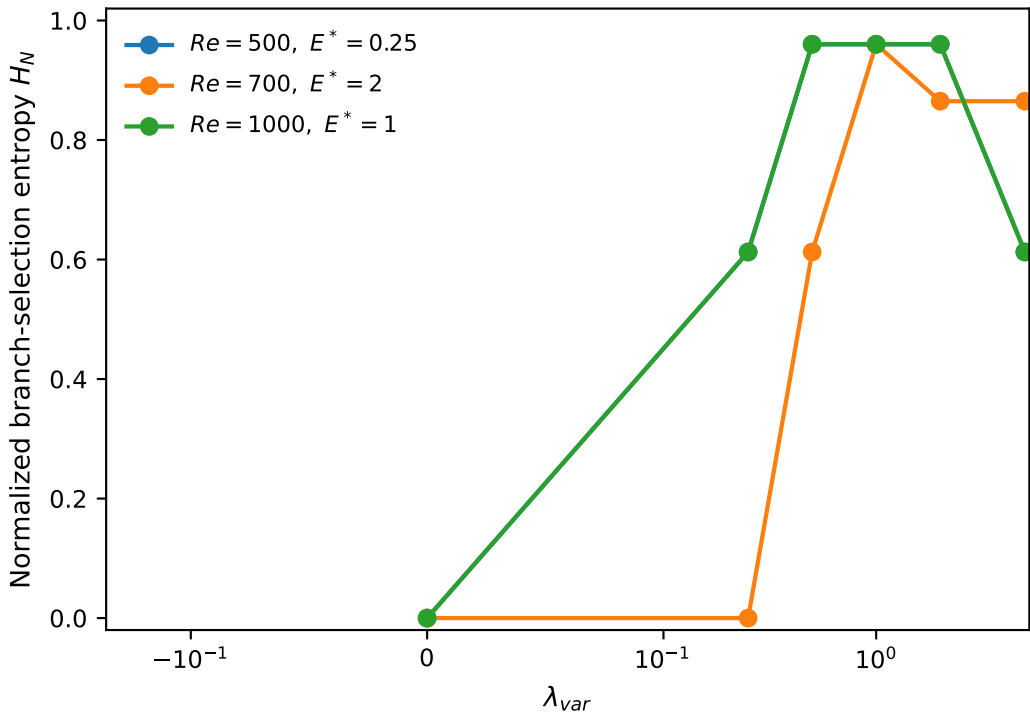
Training-output diversity as a function of the variance regularizer
