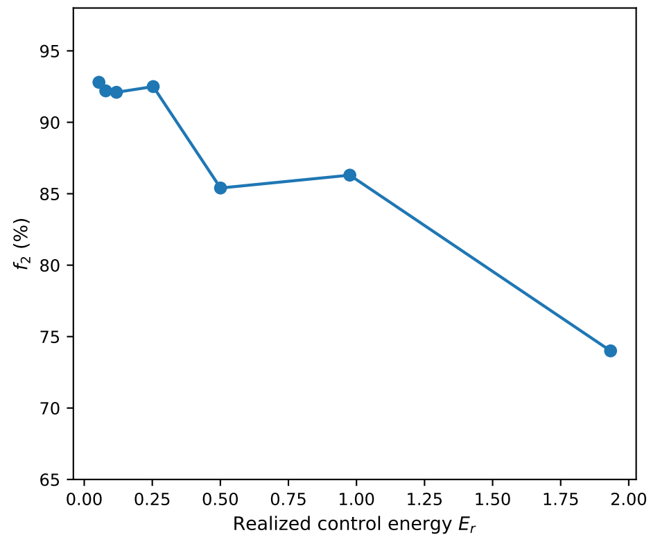
Actuation-energy dependence at Re = 500
