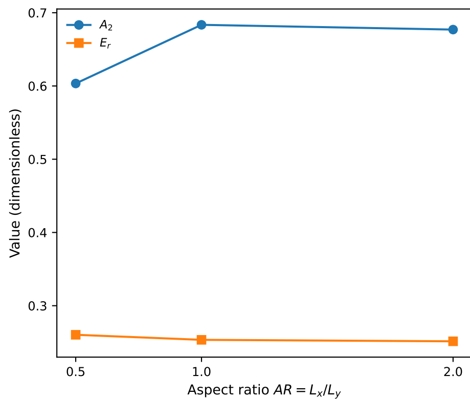
Aspect-ratio dependence at Re = 500 , E^* = 0.25
