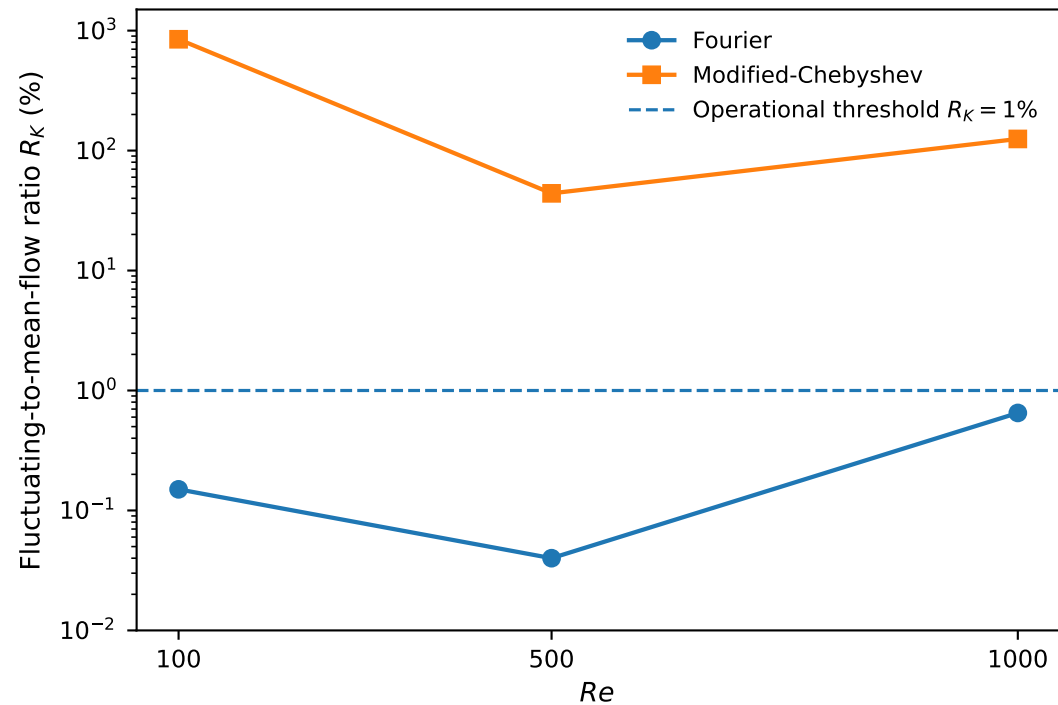
Independent LBM quasi-stationarity assessment
