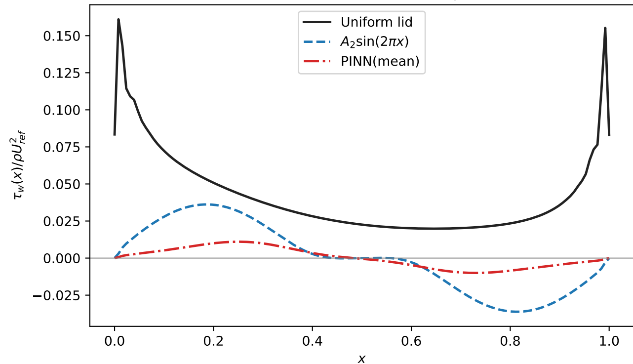
Wall shear stress at the lid ( y=1 )
