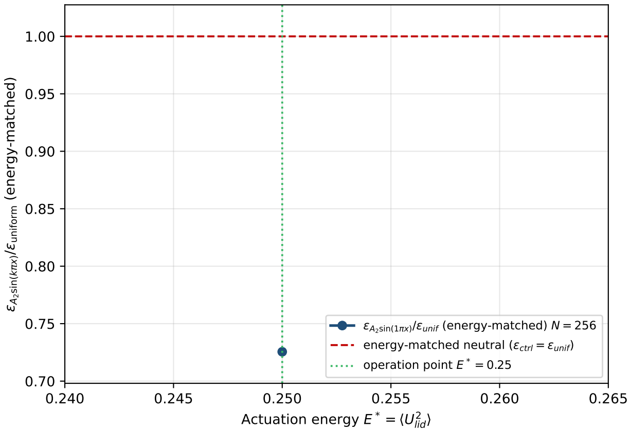
A_2 \sin(1\pi x) vs uniform lid, Re=500 , N=256
