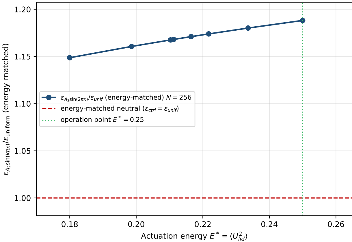
A_2\sin(2\pi x) vs uniform lid, Re=500 , N=256
