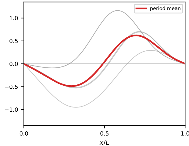
B3 (seed 0)
