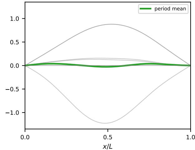
B2 (seed 5)
