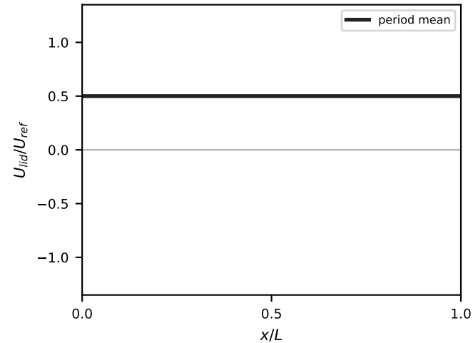
Uniform
