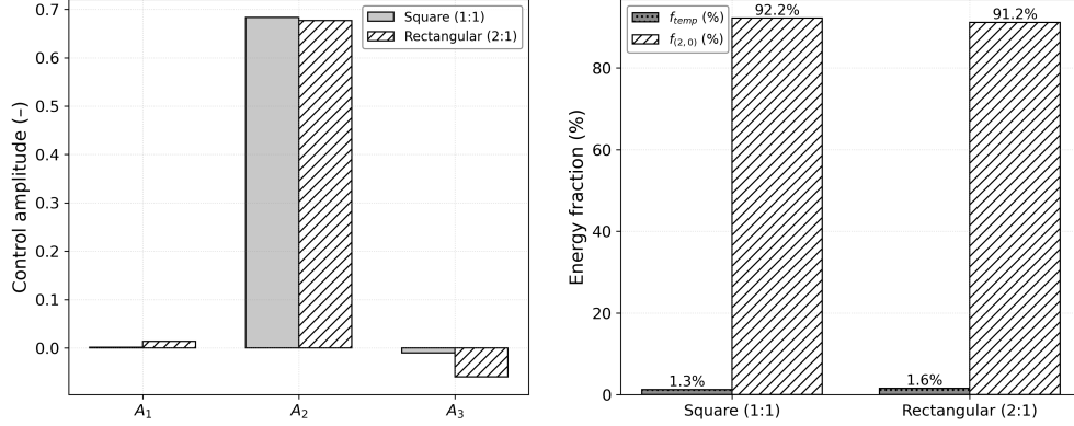
Aspect-ratio robustness (R3.2) — 1:1 vs 2:1 cavities (Re=500, seed 42): Mode-2 collapse persists Control coefficients A_i = C_{i-1,0} (-)
