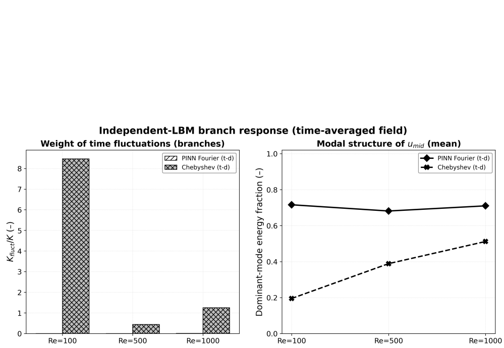
Figure 14: Global temporal behavior of the LBM realizations under all tested lid controls at Re = 100, 500 , and 1000 . The time-dependent Fourier branch (PINN t -dependent) is quasi-stationary, while the modified-Chebyshev branch remains strongly time-dependent.
