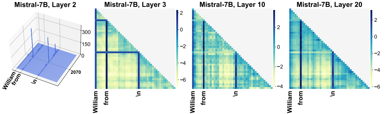
Figure 33: Average attention logits over all heads in layers 3, 10 and 20 of Mistral-7B. The input sequence is “William Shakespeare was a famous writer from England who wrote plays and poems. He is considered one of the best writers ever.\\n His works include famous plays like 'Romeo and Juliet' and 'Hamlet'.”.
