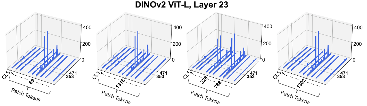
Figure 43: Illustration of massive activations in DINOv2 ViT-L for the 4 images shown in Figure 41.
