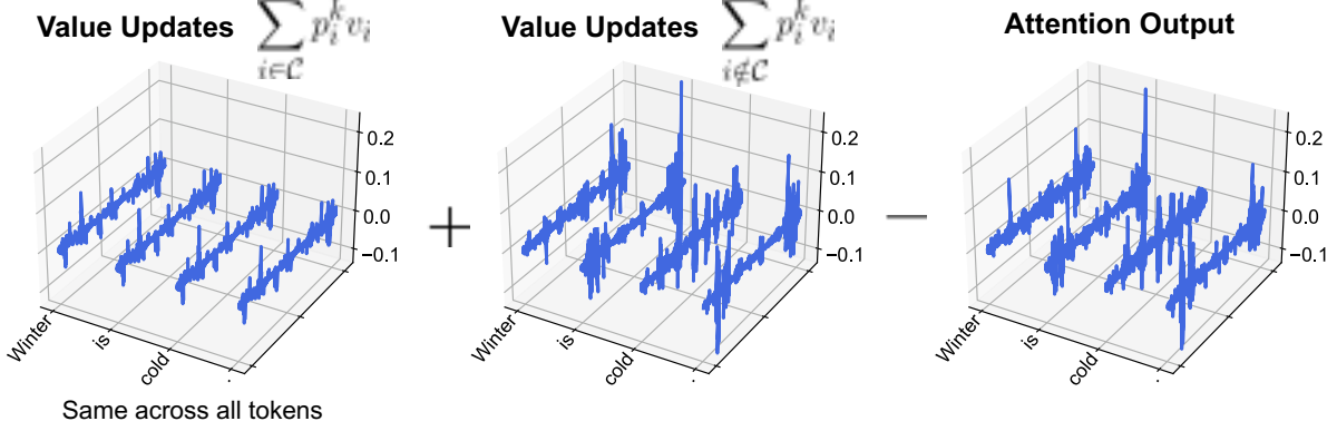
Figure 8: Value updates from tokens associated with massive activations are essentially the same.
