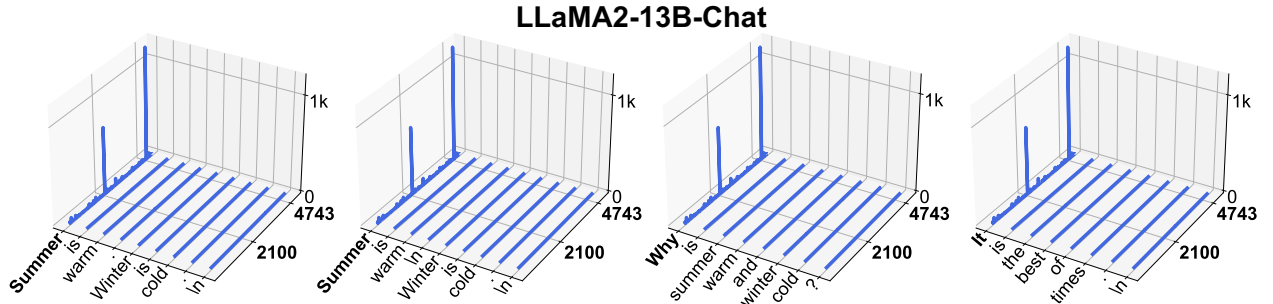
Figure 25: Massive activations in LLaMA2-13B-Chat.
