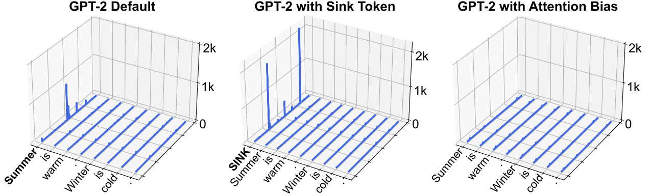
Figure 9: Massive activations disappear when training GPT-2 with explicit attention bias (Equation 3).
