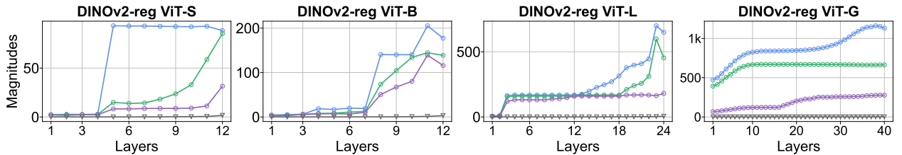
Figure 47: Layer-level analysis for ViTs in DINOv2-reg.
