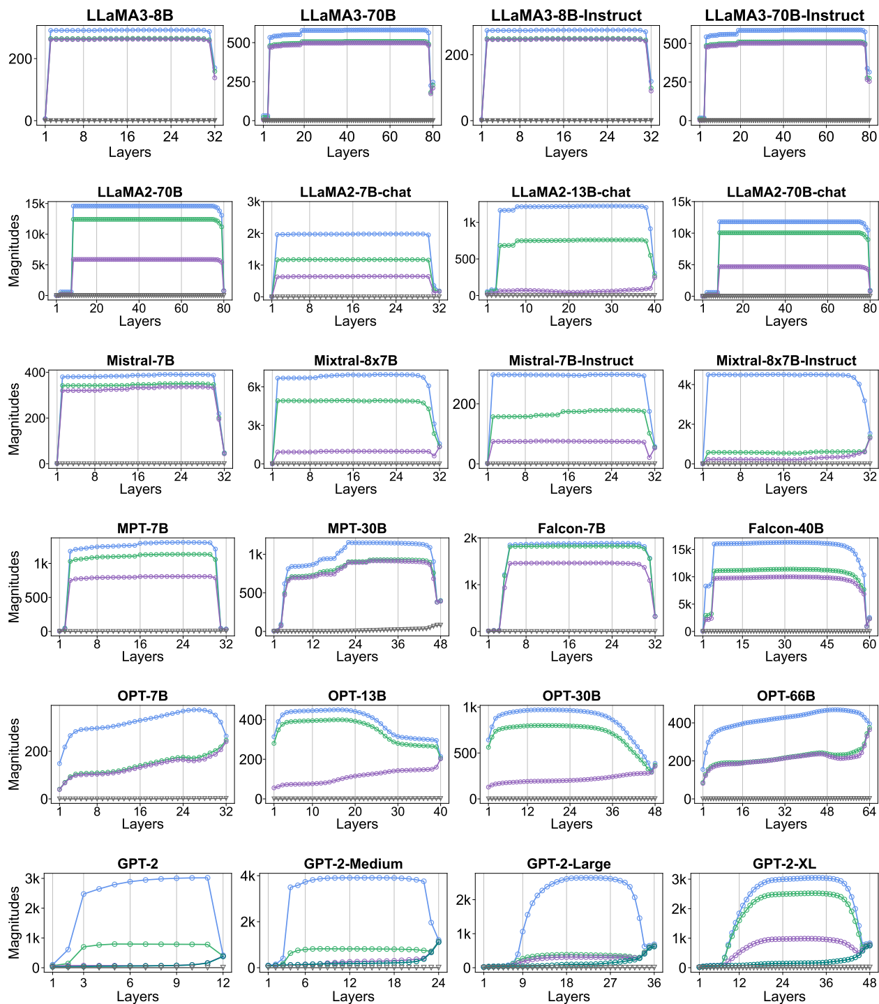
Figure 31: Layer-level analysis of LLMs. For each model, we show the three largest activation magnitudes as well as the median per layer.
