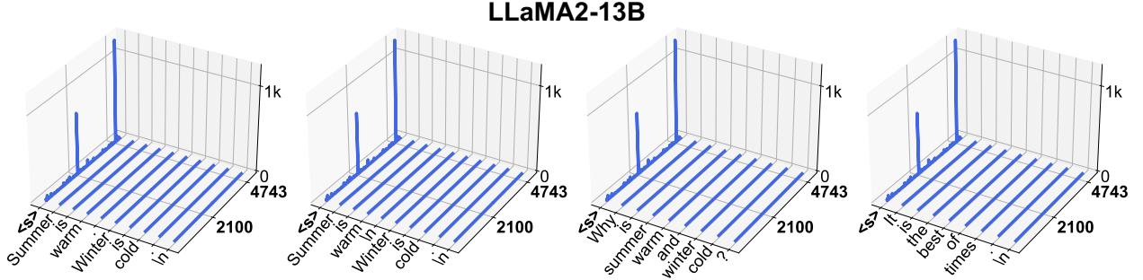
Figure 29: Massive activations in LLaMA2-13B when the input sequence is prepended with a BOS token \langle s \rangle .
