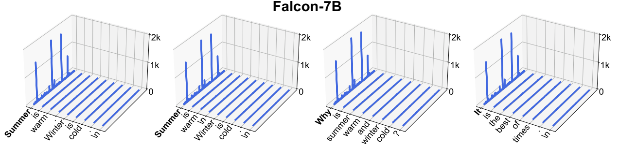
Figure 23: Massive activations in Falcon-7B.
