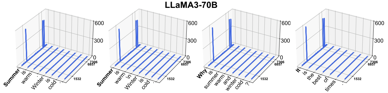
Figure 19: Massive activations in LLaMA3-70B.
