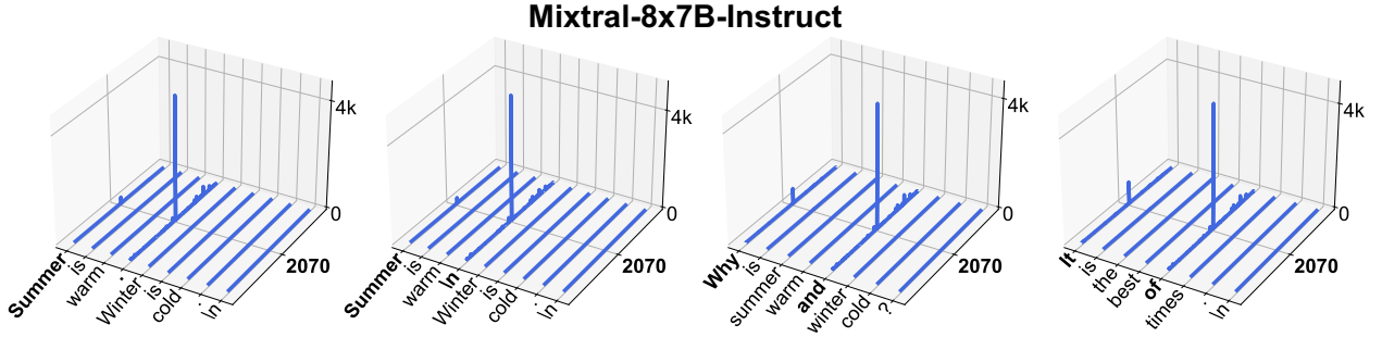
Figure 27: Massive activations in Mixtral-8x7B-Instruct.
