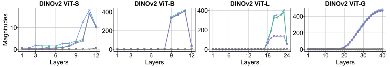
Figure 46: Layer-level analysis for ViTs in DINOv2.
