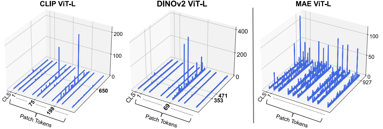
Figure 11: Massive activations are present in ViT-L from CLIP and DINOv2, but not MAE.
