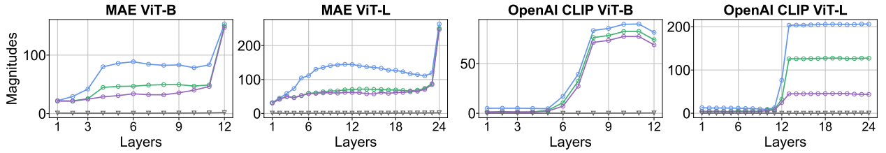
Figure 45: Layer-level analysis for ViTs in MAE and CLIP.
