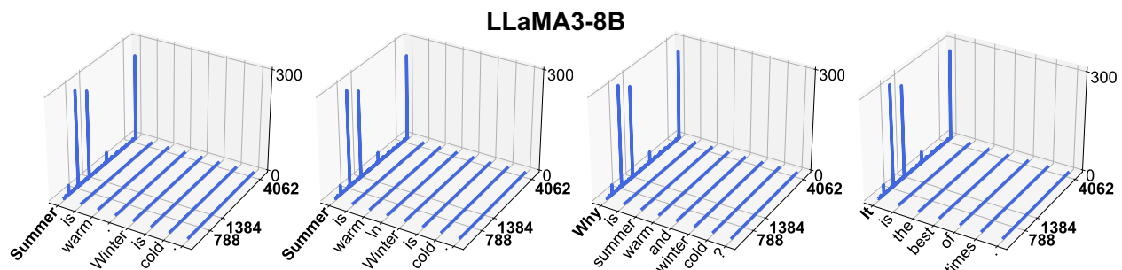
Figure 18: Massive activations in LLaMA3-8B.
