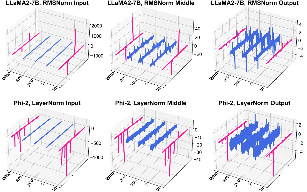
Figure 35: Activation trajectory in the attention LayerNorm of LLaMA2-7B and Phi-2, where the LayerNorm input contains massive activations. Note that LLaMA2-7B uses a variant of layer normalization: RMSNorm (Zhang and Sennrich, 2019) and Phi-2 uses the default LayerNorm (Ba et al., 2016).
