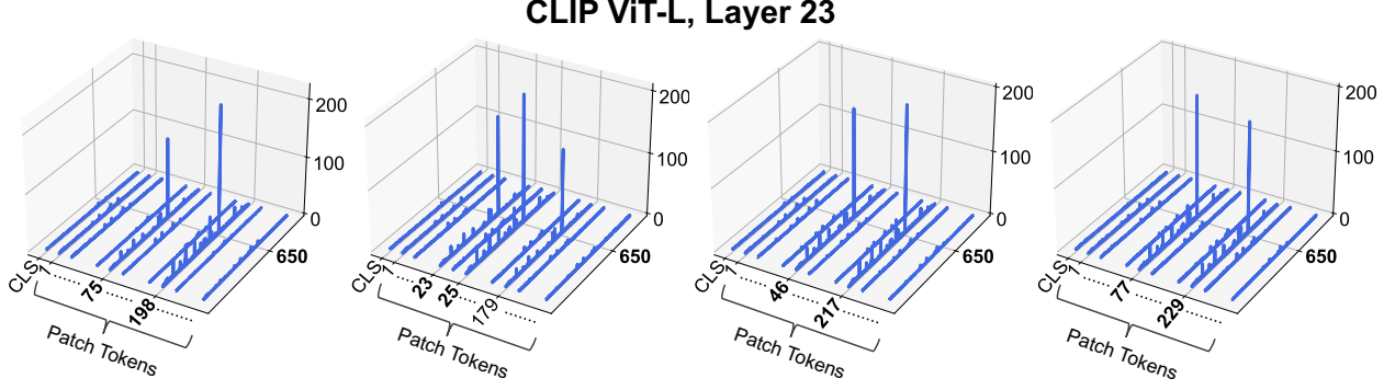
Figure 42: Illustration of massive activations in CLIP ViT-L for the 4 images shown in Figure 41.
