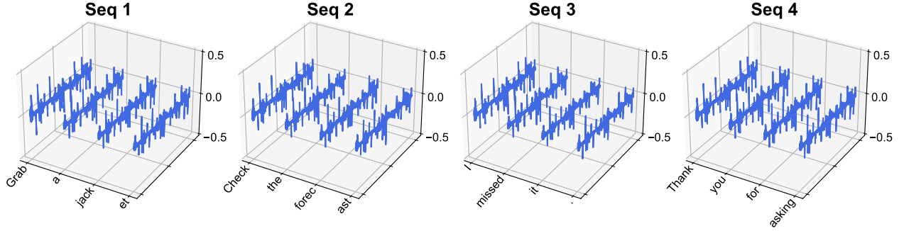
Figure 37: Value updates \sum_{i \in \mathcal{C}} p_i^k v_i at layer 15 of LLaMA2-7B, with four input sequences.
