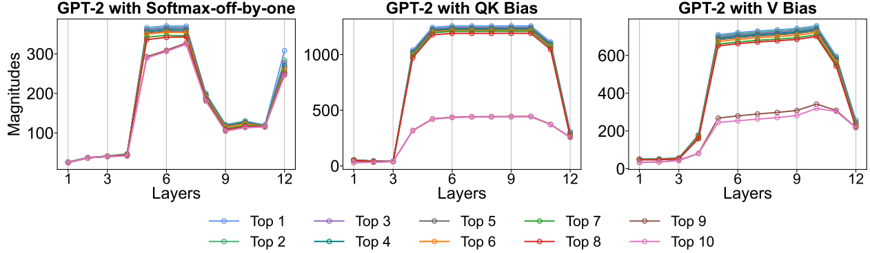
Figure 40: Ten largest activation magnitudes at each layer in three GPT-2 models.
