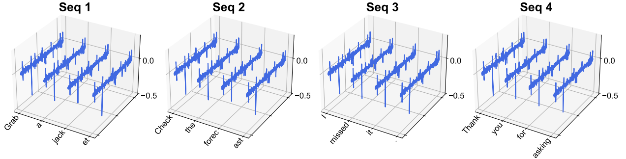
Figure 38: Value updates \sum_{i \in \mathcal{C}} p_i^k v_i at layer 30 of LLaMA2-7B, with four input sequences.
