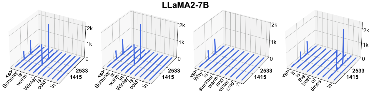
Figure 28: Massive activations in LLaMA2-7B when the input is prepended with a BOS token <s>.
