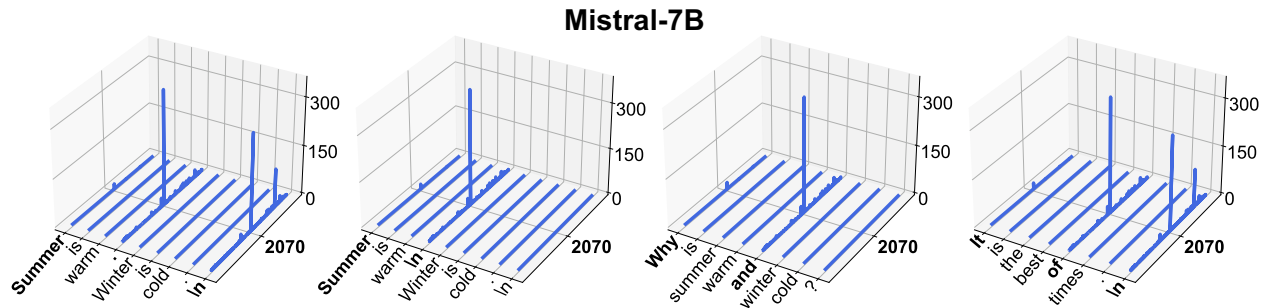
Figure 21: Massive activations in Mistral-7B.
