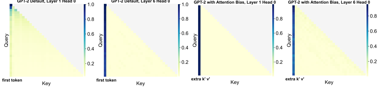
Figure 39: Attention distribution in default GPT-2 and GPT-2 with explicit attention bias.
