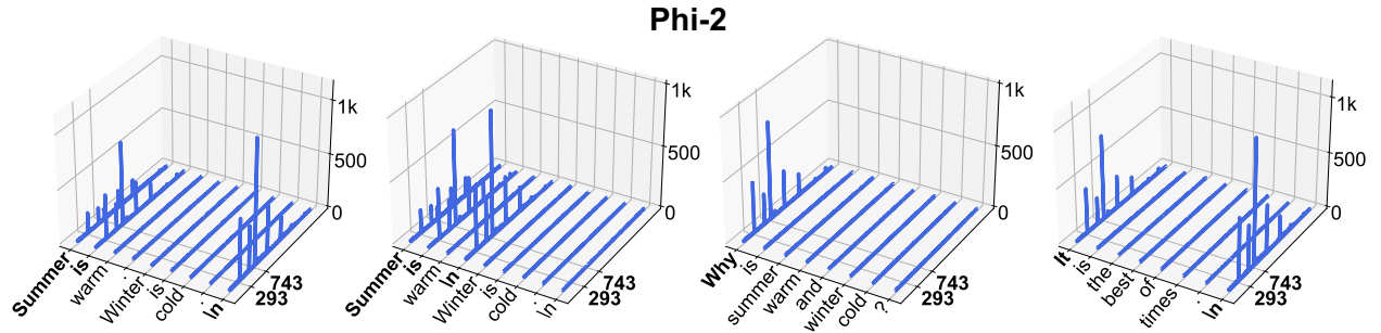
Figure 20: Massive activations in Phi-2.
