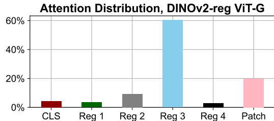
Figure 16: Average attention of the [CLS] token.
