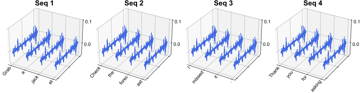
Figure 36: Value updates \sum_{i \in \mathcal{C}} p_i^k v_i at layer 3 of LLaMA2-7B, with four input sequences.
