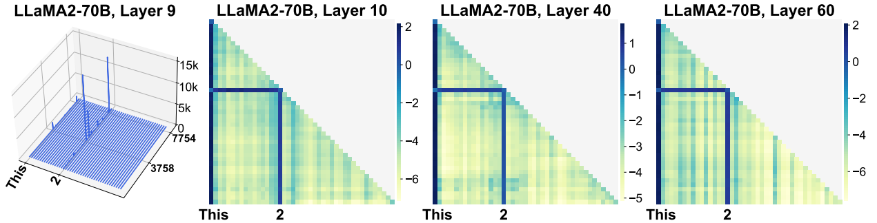
Figure 32: Average attention logits over all heads in layers 10, 40 and 60 of LLaMA2-70B. The input sequence is “This book, including all illustrations and text, is protected under Copyright©2024 and may not be reproduced or transmitted in any form without the prior written permission of the copyright owner.”.
