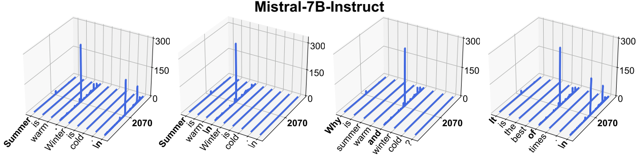
Figure 26: Massive activations in Mistral-7B-Instruct.
