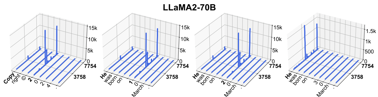
Figure 17: Massive activations in LLaMA2-70B.
