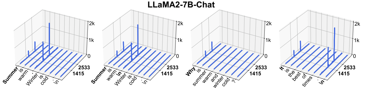
Figure 24: Massive activations in LLaMA2-7B-Chat.
