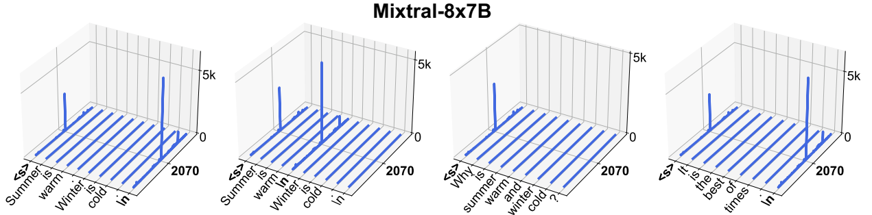
Figure 30: Massive activations in Mixtral-8x7B when the input sequence is prepended with a BOS token \langle s \rangle .
