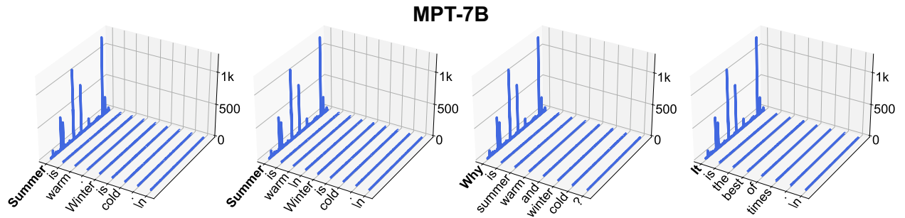
Figure 22: Massive activations in MPT-7B.
