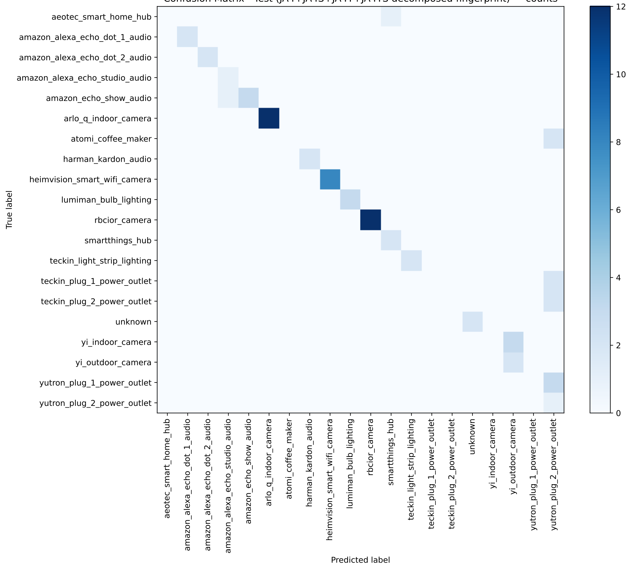
Confusion Matrix - Test (JA4+JA4S+JA4T+JA4TS decomposed fingerprint) — counts
