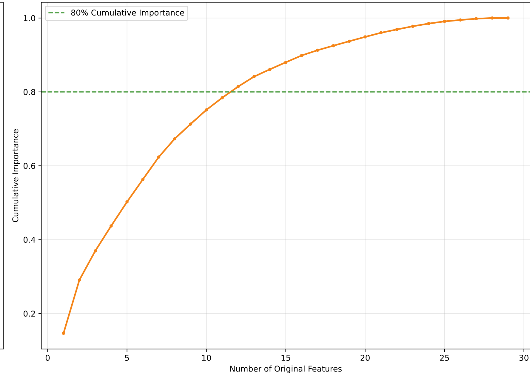
Cumulative Importance by Original Feature
