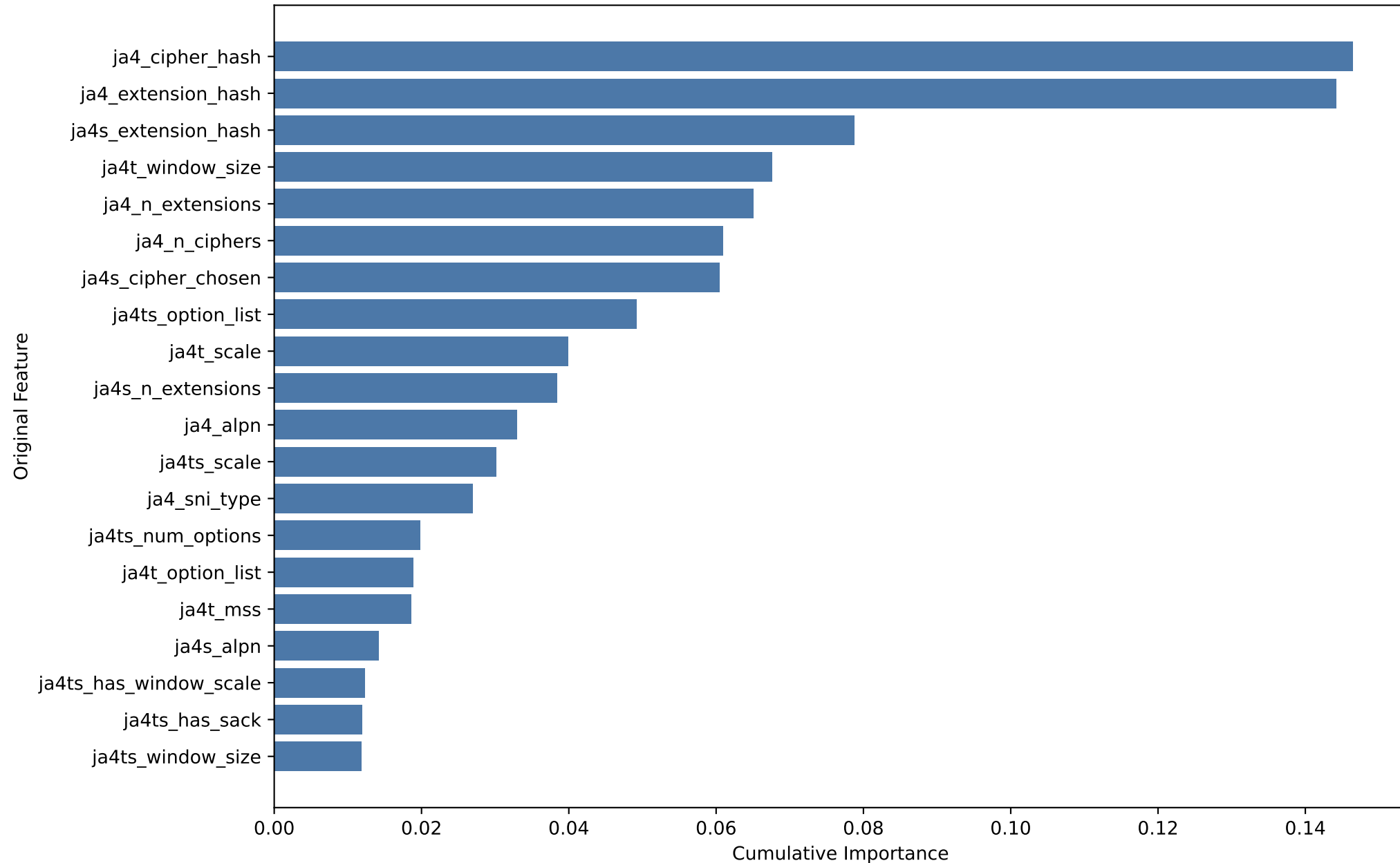
Top 20 Most Important Original Features
