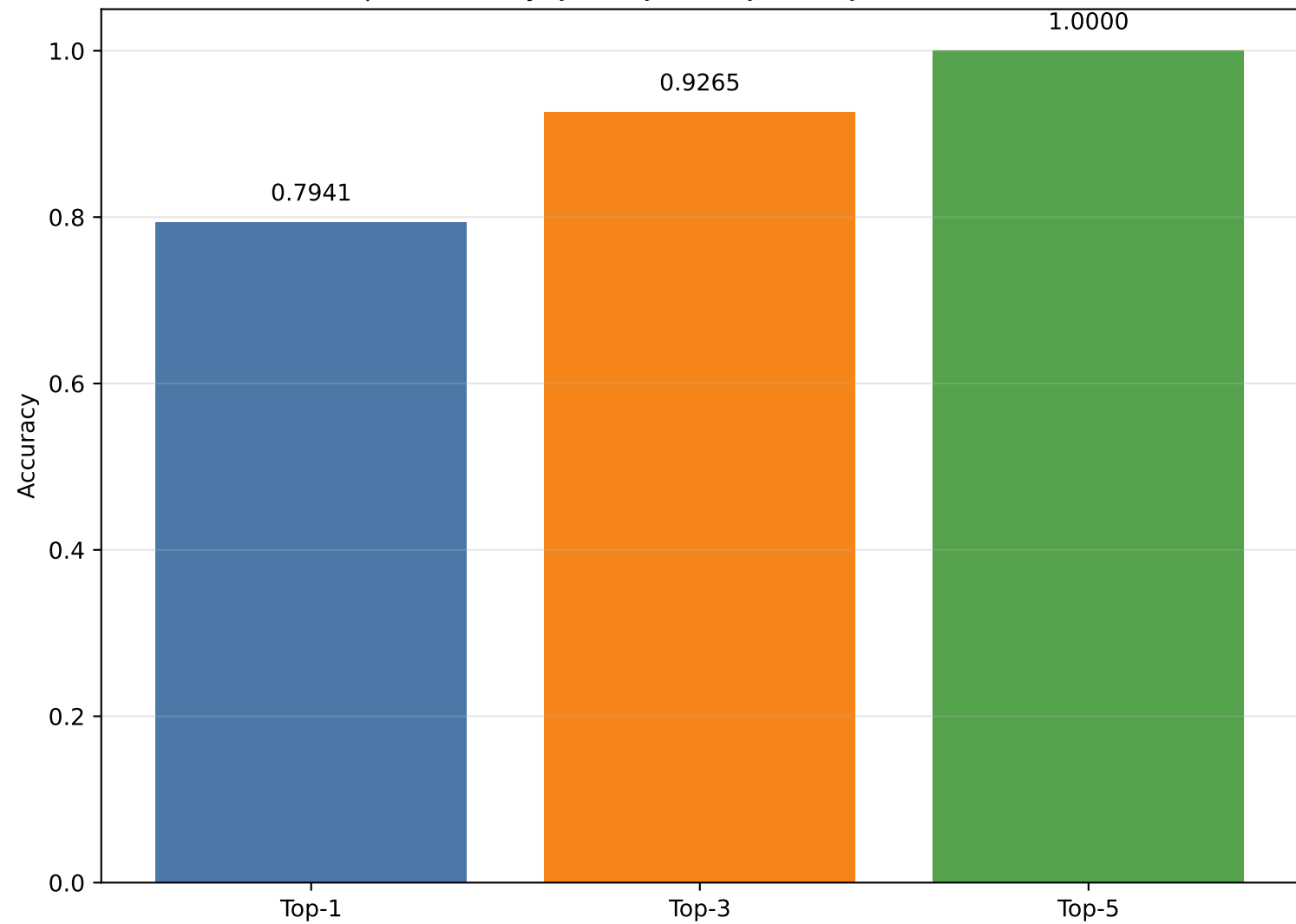
Top-k accuracy (JA4 + JA4S + JA4T + JA4TS features)
