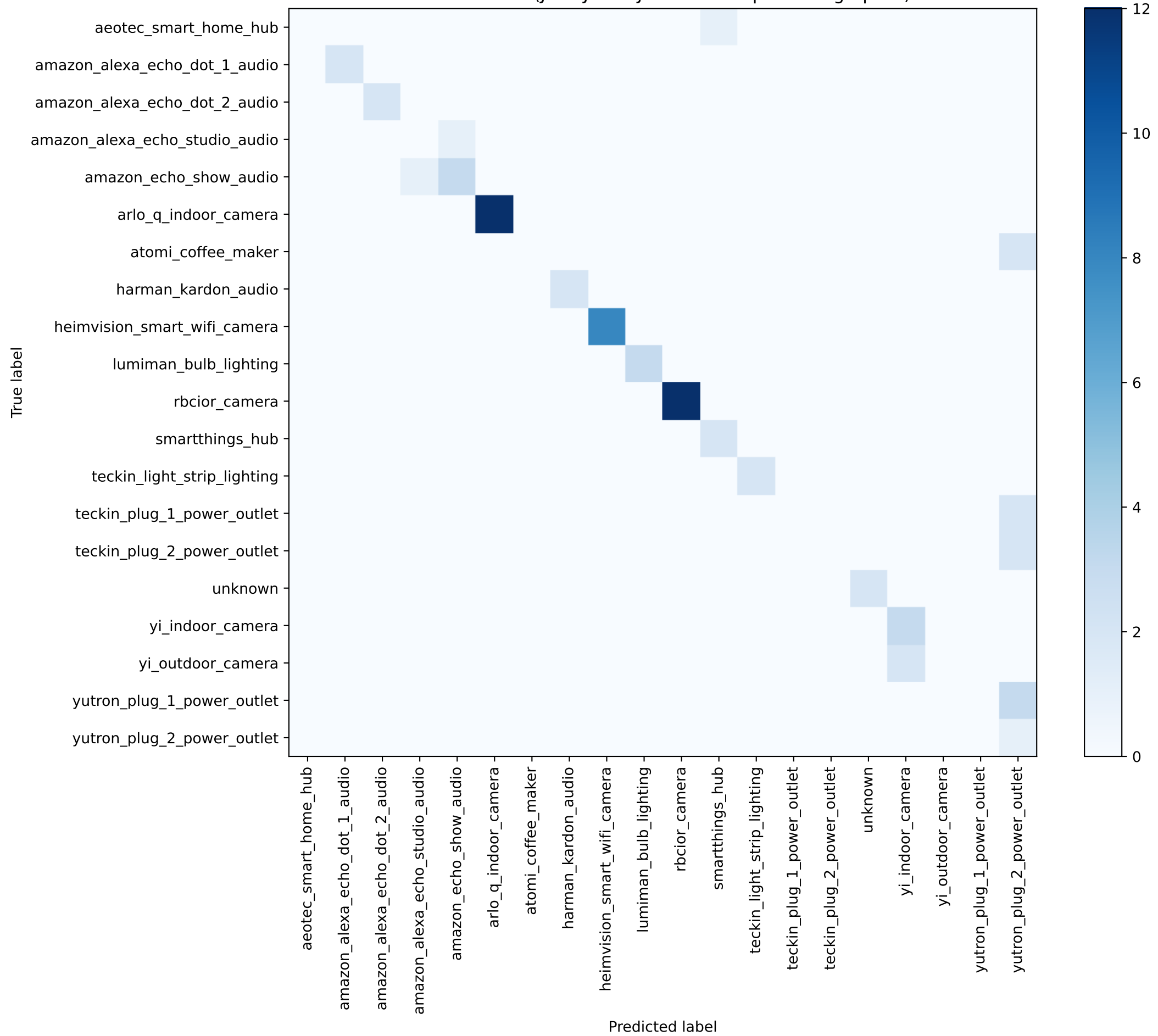
Confusion Matrix - Test (JA4+JA4S+JA4TS decomposed fingerprint) — counts
