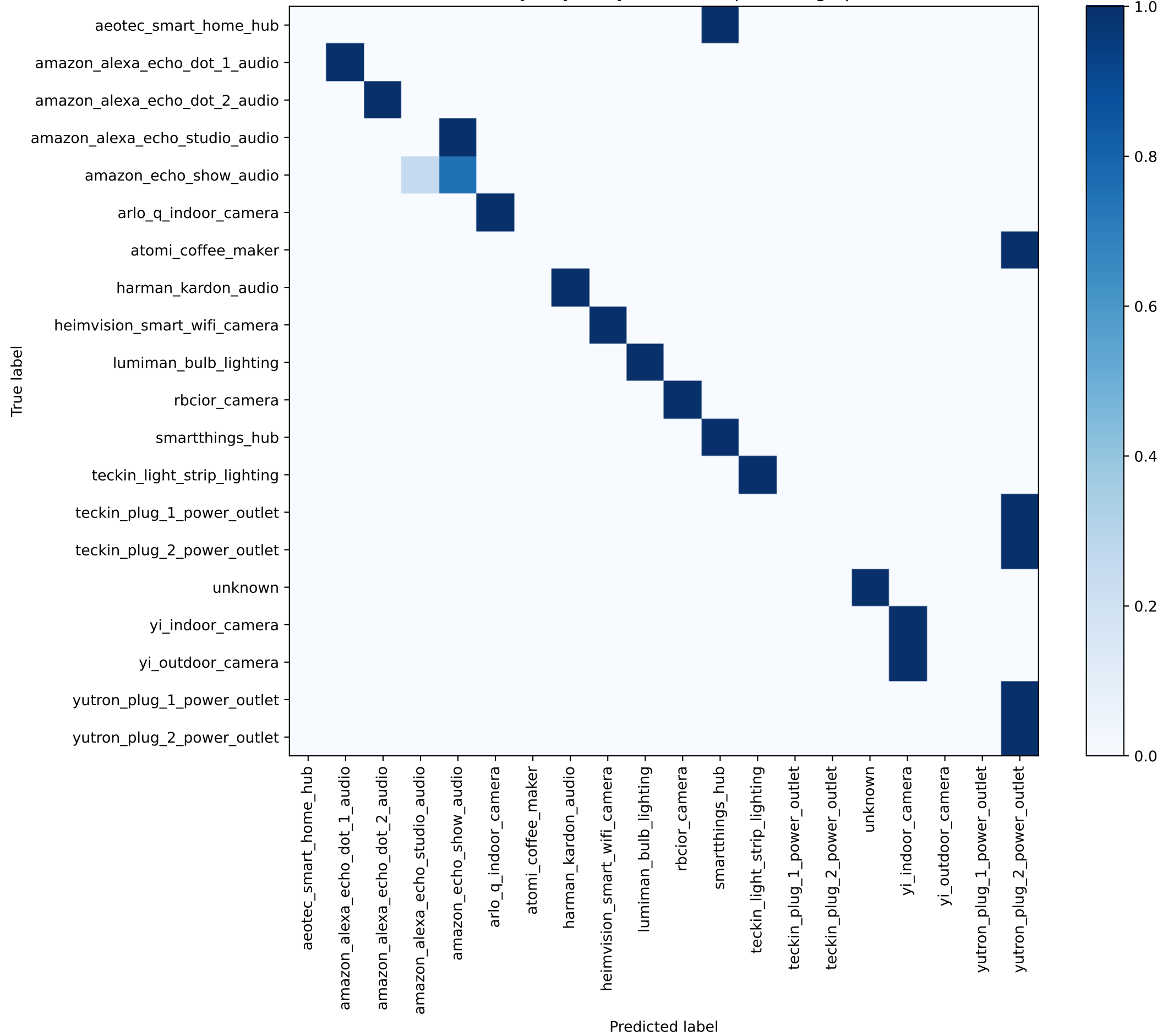
Confusion Matrix - Test (JA4+JA4S+JA4TS decomposed fingerprint) — normalized
