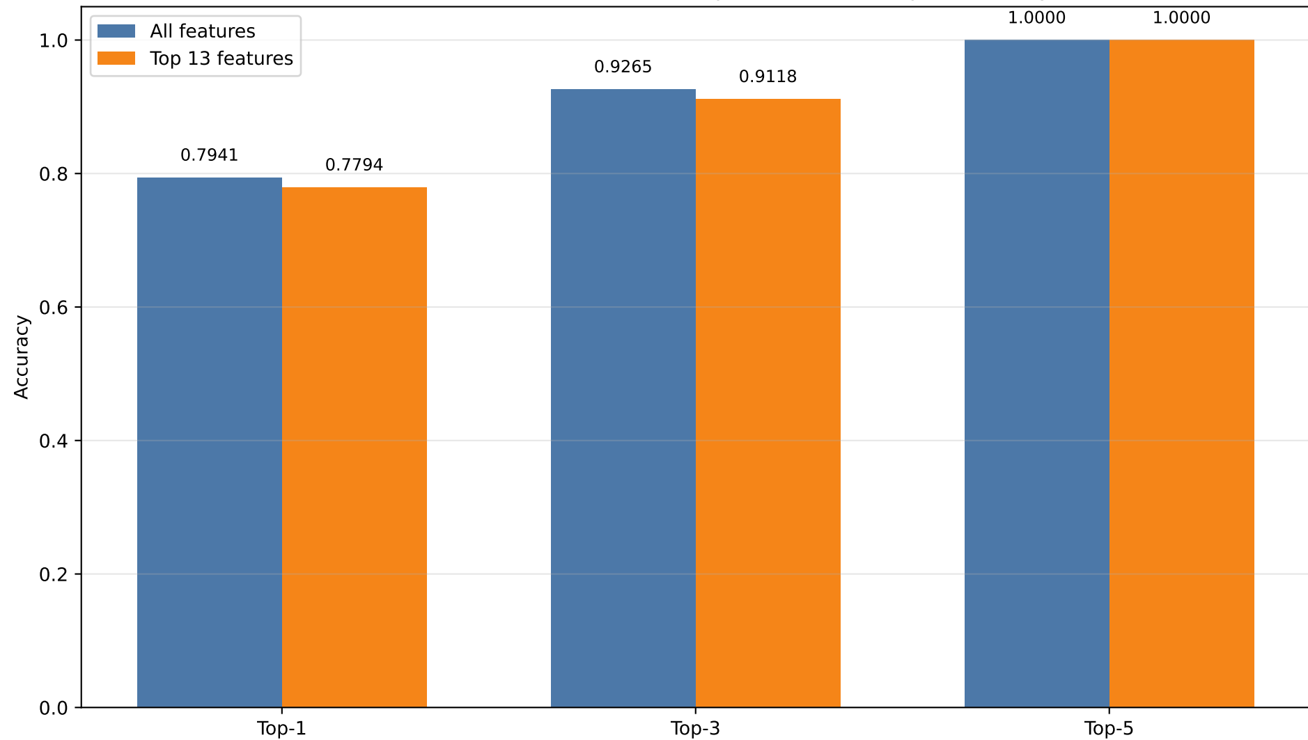
JA4 + JA4S + JA4TS features vs Top 13 features - Top-k accuracy
