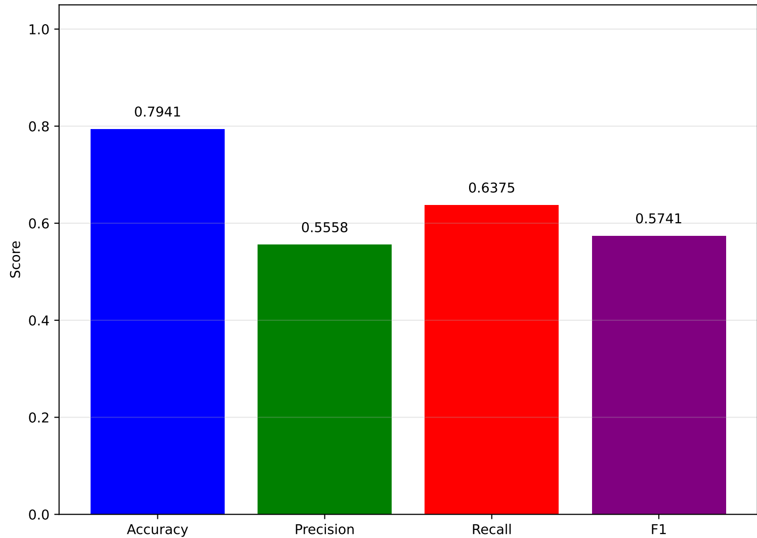
Test Metrics (JA4 + JA4S + JA4TS features)
